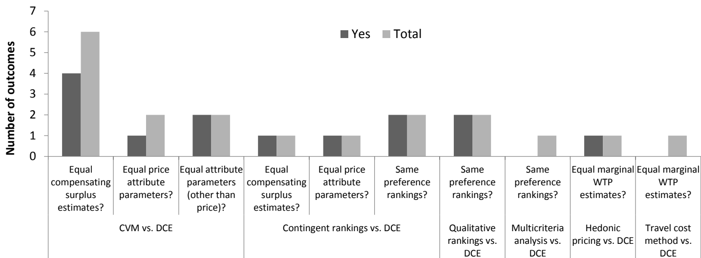
Figure 5: Convergent validity tests: Does DCE produce the same results as other methods?
