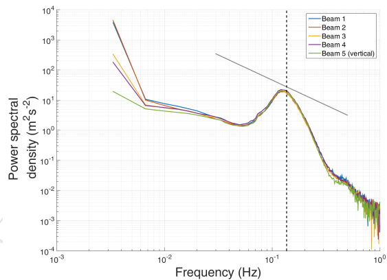
Figure 14: Mean power spectral densities across the whole ADCP record for each of the five beams; each coloured line corresponds to a different beam. Grey line shows the expected -5/3 slope, and dotted black line shows the median wave period during the ADCP deployment.
