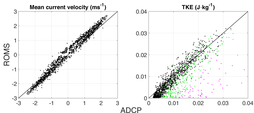
Figure 8: Scatter plots comparing measured data from ADCP and predictions from ROMS. Left-hand panel shows mean current velocities; right-hand panel shows mean TKE for the lower half of the water column. In the TKE comparison, magenta points are excluded if the 95 th %ile criterion for waves is applied; if the 75 th %ile criterion is applied, the green points are also excluded.
