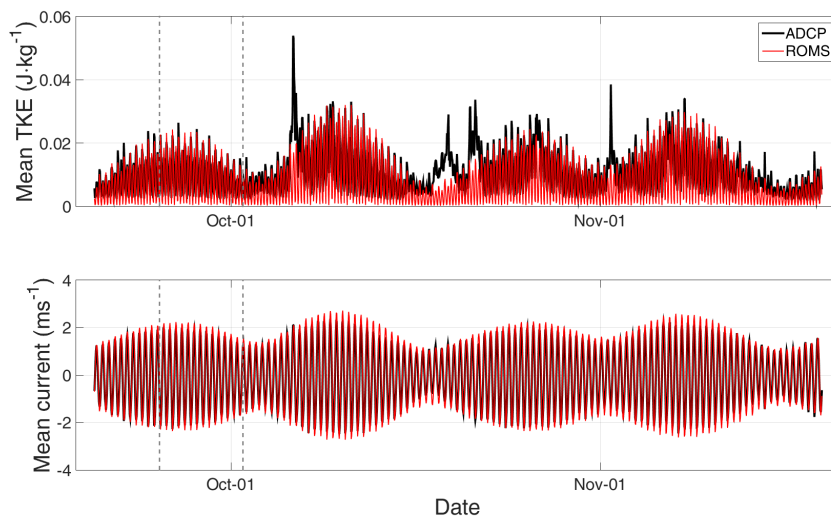
Figure 4: Comparison of ADCP and ROMS results over the time period of the ADCP deployment. Upper panel shows time series of vertical-mean TKE from the lower half of the water column. Lower panel shows mean current velocities; flood velocities are shown as positive and ebb velocities as negative. Dashed grey lines indicate the subset shown in more detail in figure 5
