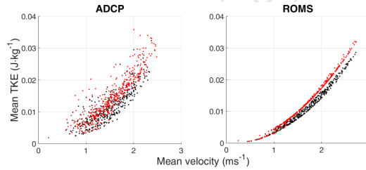
Figure 6: Scatter plot comparing mean flow and TKE for ADCP measurements (left panel) and ROMS estimates (right panel). Black points correspond to flood phases, red points to ebb phases.
