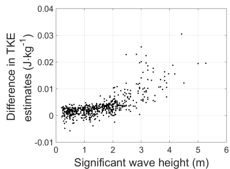
Figure 13: Scatter plot visualising the effect of wave height as measured by buoy on difference in TKE density from ADCP measurements and ROMS estimates.
