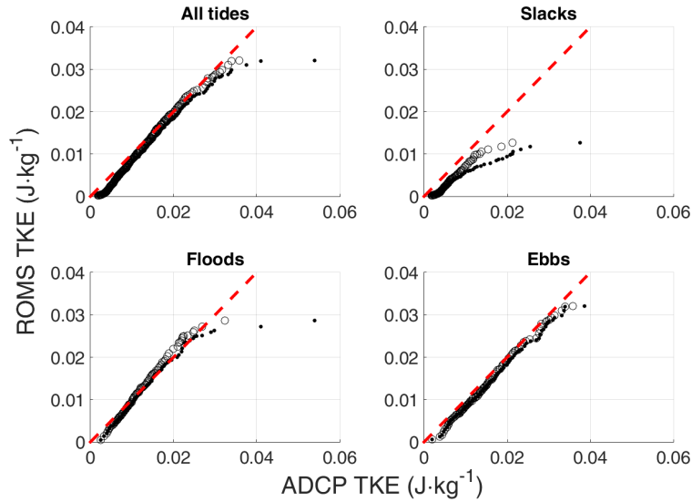
Figure 10: Comparison of TKE probability distributions between ROMS simulation and ADCP measurements visualised as q-q plots. Dots show the quantiles for the complete data set, circles show quantiles for the data set with the 95 th %ile condition on waves applied; the line of equality is shown as red dashes. To improve legibility, only every fifth quantile has been plotted.
