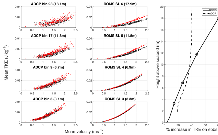
Figure 7: Scatter plot comparing mean flow velocity and TKE at four depths for ADCP measurements (left column) and ROMS estimates (central column). Black points correspond to flood phases, red points to ebb phases. Right column shows a profile of flood-ebb asymmetry as a percentage increase in TKE density from flood to ebb. Circles indicate the depths from which the data in scatter plots are taken.
