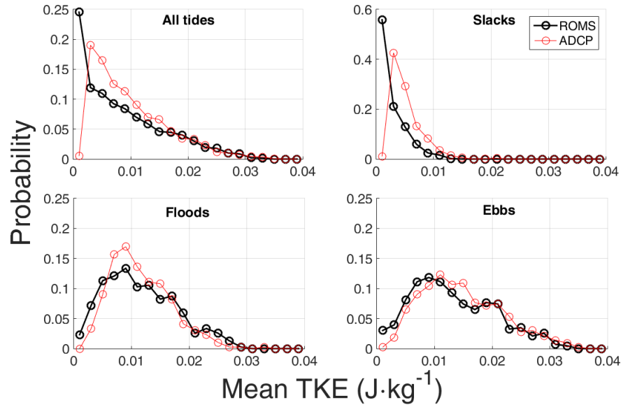
Figure 9: Comparison of probability distributions of mean TKE for the lower half of the water column taken from ROMS simulation and ADCP data.
