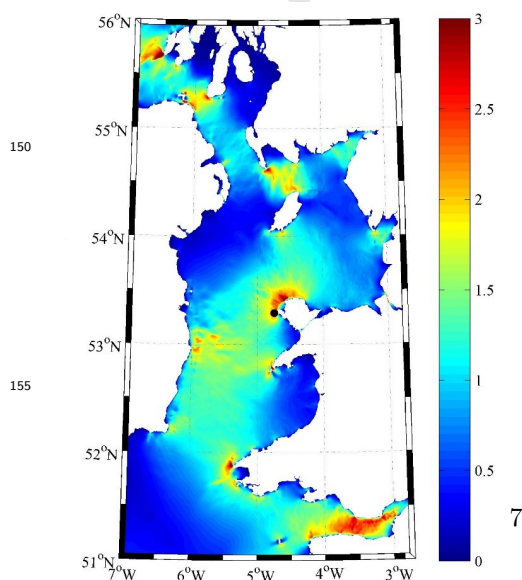
Figure 2: Map of ROMS model area domain. Contours show depth-averaged peak spring tidal current in \text{ms}^{-1} , as measured by the
