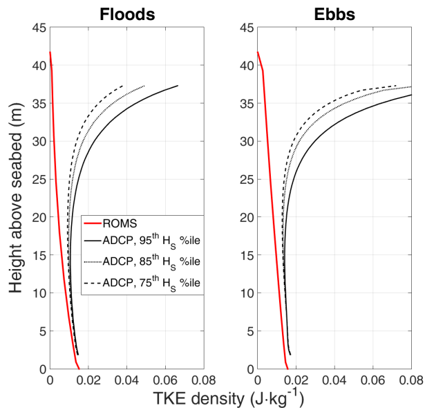
Figure 11: Vertical profiles of TKE density for ROMS results and ADCP data. Different ADCP profiles correspond to different wave conditions. The 95 th %ile wave ADCP profile uses only data from times during which H_S did not exceed the 95 th percentile to calculate the mean; a similar condition applies for the 85 th %ile and 75 th %ile profiles.
