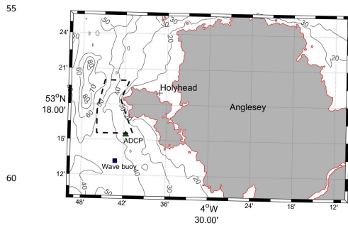
Figure 1: Location of West Anglesey Demonstration Zone off the coast of Anglesey, marked with black dashed line. Bathymetry contours 65 show depth relative to mean sea level.
