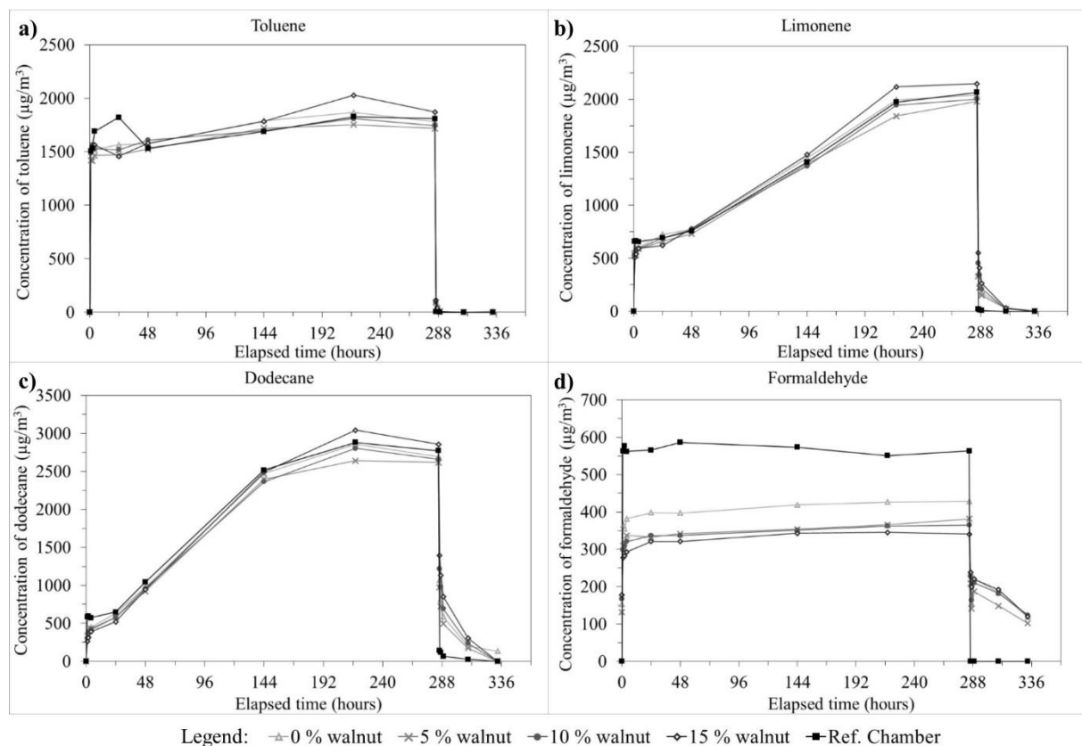
Figure 8. Adsorption/desorption curves of a) toluene, b) limonene, c) dodecane and d) formaldehyde.
