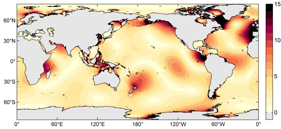
Figure 1. M_2 RMS elevation error (cm) between the TPXO8 atlas and our \frac{1}{12}^\circ simulations based on online evaluation of SAL and a scale factor of \kappa_w = 0.3 applied to the conversion scheme. Corresponding global-mean RMS errors are 4.4 cm for depths greater than 1000 m and 14.6 cm in shallow oceans.
