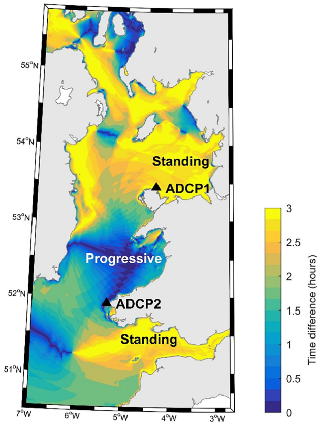
Fig. 4. Time difference ( \Delta T in hours) between high water and peak M_2 current speeds in the Irish Sea. \Delta T is given as coloured contours in 10-min intervals. Black triangles show the locations of ADCP1 and ADCP2.
