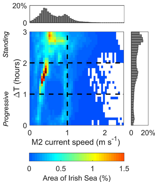
Fig. 5. Colour matrix showing areal extent of the Irish Sea (%), distributed in terms of peak depth-averaged M_2 current speeds and standing/progressive wave systems. The top panel shows the distribution in terms of peak M_2 current speeds only (i.e. summing the matrix columns). The right panel shows the distribution in terms of the nature of the wave system only (i.e. summing the matrix rows). As an example interpretation, the majority of the Irish Sea experiences standing wave systems ( \Delta T > 2 h) with peak M_2 current speeds less than 1 m/s. The vertical dashed black line highlights M_2 current speeds > 1 m/s (regarded as a minimum threshold for tidal stream sites) and the horizontal dashed black lines differentiate between standing, partially-progressive and progressive wave systems. (For interpretation of the references to color in this figure legend, the reader is referred to the web version of this article.)
