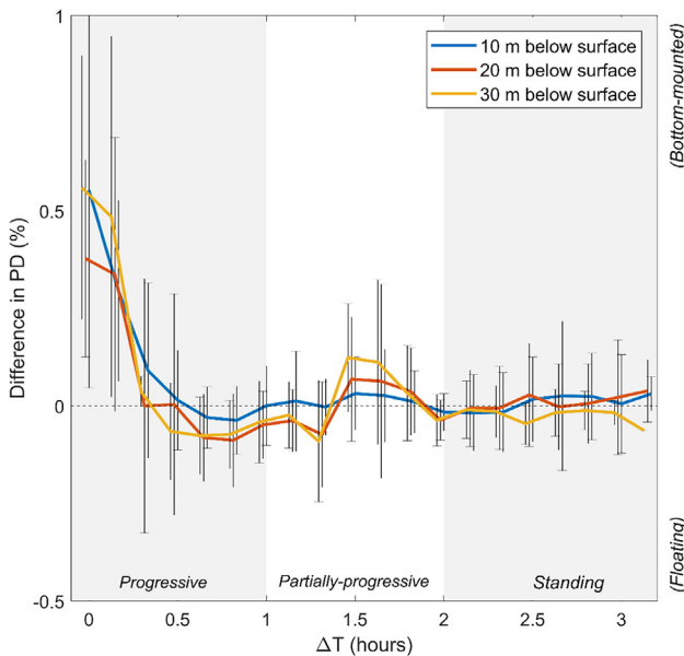
Fig. 11. Relationship between the nature of the tidal wave ( \Delta T ) and percentage difference in power density, for three different depths below surface. The analysis corresponds to regions of the Irish Sea model where simulated depth-averaged M 2 flow exceeds 1 m/s. Error bars denote one standard deviation from the mean. Positive percentage differences in power density indicate greater energy available for extraction by bottom-mounted devices than by floating devices at that depth below surface, and vice versa.
