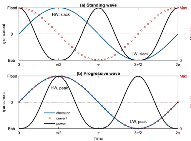
Fig. 2. Phase relationship between tidal elevations (blue line) and tidal currents (red circles), for (a) standing and (b) progressive wave systems. Also shown is the power density (black lines), approximated using the absolute value of the velocity cubed, U^3 , see Eq. (2)). Note the different scales on the left- and right axes. (For interpretation of the references to color in this figure legend, the reader is referred to the web version of this article.)
