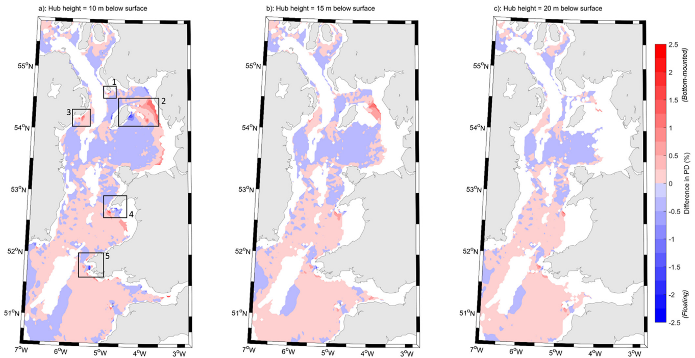
Fig. 9. Difference (in %) of power density (in \text{kW/m}^2 ) between floating and bottom-mounted tidal stream devices, calculated using simulated tidal current speeds over a 30 day period throughout the Irish Sea. Panel (a) compares flows encountered by a floating device (10 m below the changing sea surface) with flows encountered by a bottom-mounted device (10 m below the fixed mean sea level). Panels (b) and (c) show similar comparisons at 15 m and 20 m depths below surface. Deep water ( > 100 m) and shallow water ((a) < 20 m, (b) < 30 m, (c) < 40 m) were not analysed (white regions).
