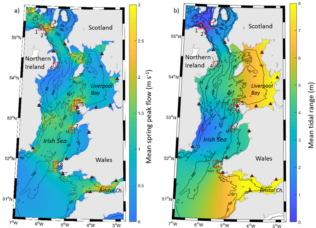
Fig. 3. Domain extent of the Irish Sea model. Colour scale in (a) shows the mean spring peak depth-averaged velocities, and in (b) shows mean tidal range. Contour lines show bathymetry at mean sea level. Existing and proposed tidal stream projects are marked (red squares): (1) Fair Head; (2) Torr Head; (3) Mull of Kintyre; (4) Strangford Lough; (5) Anglesey-Skerries; (6) Anglesey Demonstration Zone; (7) Llyn Peninsula; (8) Ramsey Sound. Tide gauge [34] locations used for validation are also marked (red triangles). (For interpretation of the references to color in this figure legend, the reader is referred to the web version of this article.)
