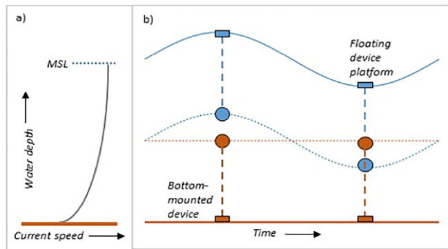
Fig. 1. (a) Schematic of a typical vertical current velocity profile. (b) Schematic showing different configurations of floating-platform (blue) and bottom-mounted (red) turbines in the water column. The hub height of the floating turbine varies with sea surface height, hence potentially experiencing a greater range of velocities than the bottom-mounted turbine.
