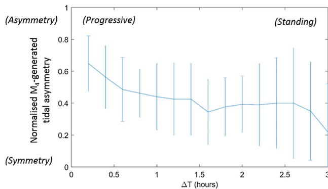
Fig. 7. Relationship between standing and progressive wave systems ( \Delta T , averaged for 12 min bins) and M_4 -generated tidal asymmetry, for locations in the Irish Sea where peak M_2 velocities exceeded 1 m/s. Tidal asymmetry was calculated based on the relationship 2\phi(M_2) - \phi(M_4) , where \phi is the tidal phase. The Y-axis has been normalised so that zero signifies tidal symmetry and one signifies maximal tidal asymmetry; see Robins et al. [3] for further details. Error bars denote one standard deviation from the mean.
