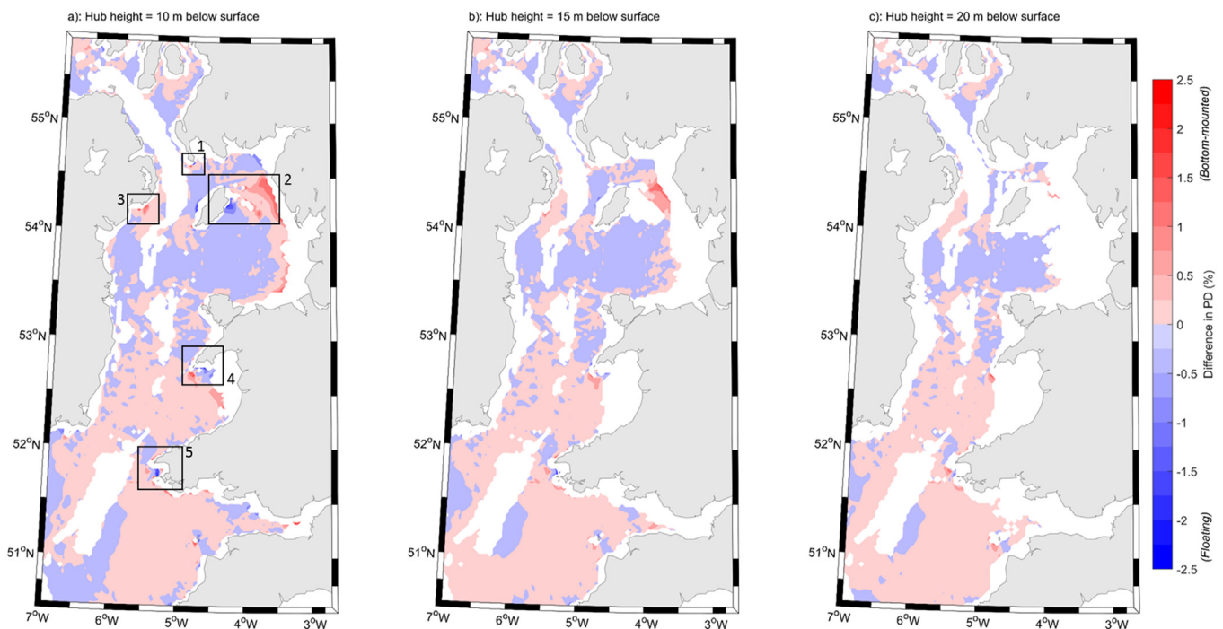
Fig. 9. Difference (in %) of power density (in \text{kW}/\text{m}^2 ) between floating and bottom-mounted tidal stream devices, calculated using simulated tidal current speeds over a 30 day period throughout the Irish Sea. Panel (a) compares flows encountered by a floating device (10 m below the changing sea surface) with flows encountered by a bottom-mounted device (10 m below the fixed mean sea level). Panels (b) and (c) show similar comparisons at 15 m and 20 m depths below surface. Deep water ( > 100 m) and shallow water ((a) < 20 m, (b) < 30 m, (c) < 40 m) were not analysed (white regions).
