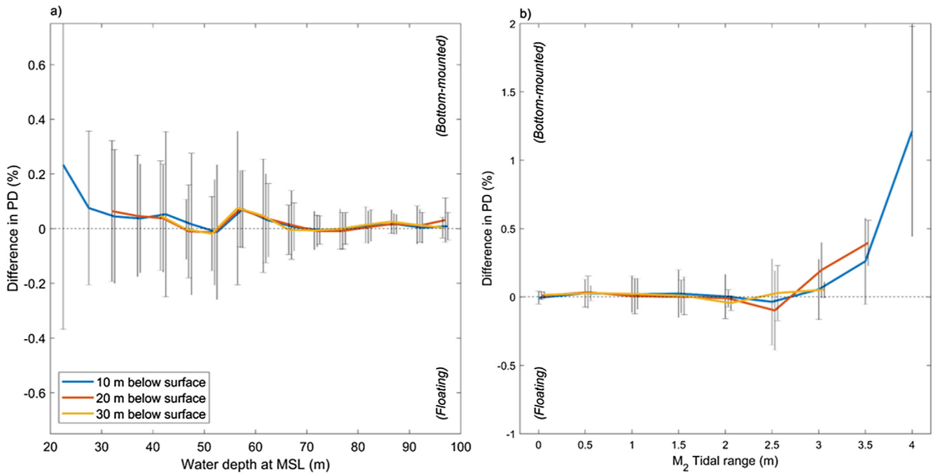
Fig. 10. Relationships between (a) water depth and percentage difference in power density (PD), and (b) tidal range and percentage difference in power density, for three different depths below the surface. The analysis corresponds to regions of the Irish Sea model where simulated depth-averaged M 2 flow exceeds 1 m/s. Error bars denote standard deviation from the mean. Positive percentage differences in power density indicate greater energy available for extraction by bottom-mounted devices than by floating devices at that depth below surface, and vice versa.
