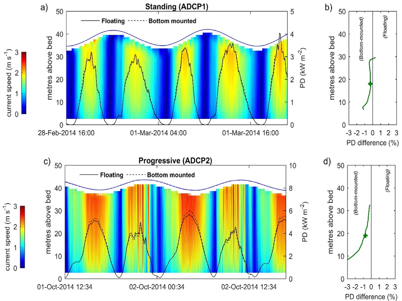
Fig. 8. Time series of observed tidal current speeds and elevations during spring tides at (a) ADCP1 (standing wave) and (c) ADCP2 (progressive wave). The black lines on the timeseries indicate the power density (right axis) calculated at the mid-depth for floating (solid) and bottom-mounted (dashed) devices. The right two panels indicate the percent difference in power density (PD) at (b) ADCP1 and (d) ADCP2, varying with water depth, where negative/positive difference in PD indicates bottom-mounted/floating devices favoured, respectively.
