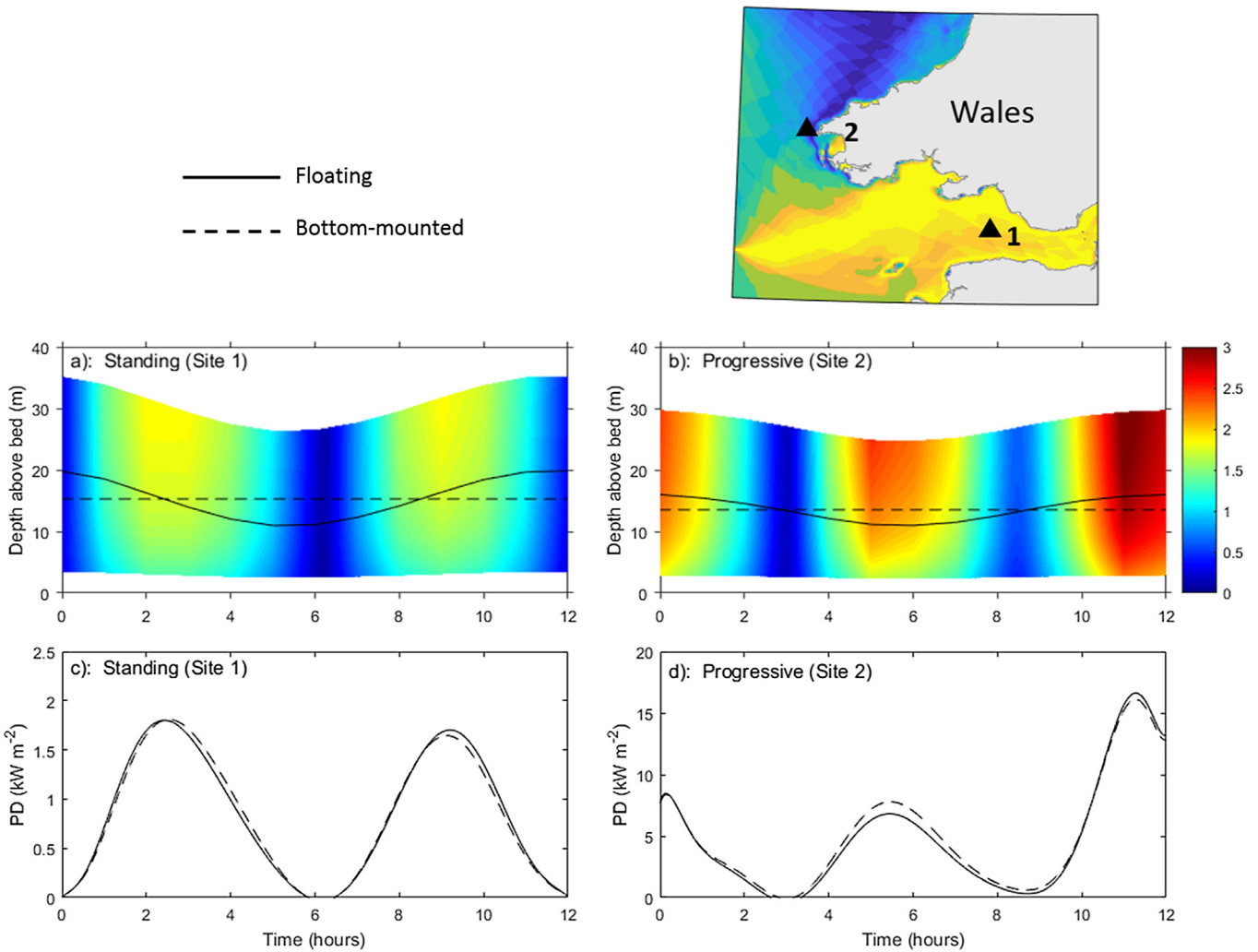
Fig. 6. Time series of simulated tidal current speeds and elevations at (a) Site 1 (standing wave) and (b) Site 2 (progressive wave). The location of these time series is plotted in the top right panel (see Fig. 4 for reference). Panels (a) and (b) also show the mid-depth position of a potential bottom-mounted device (dashed black line) and floating device (solid black curve). The power density along these lines is plotted in (c) and (d), respectively.
