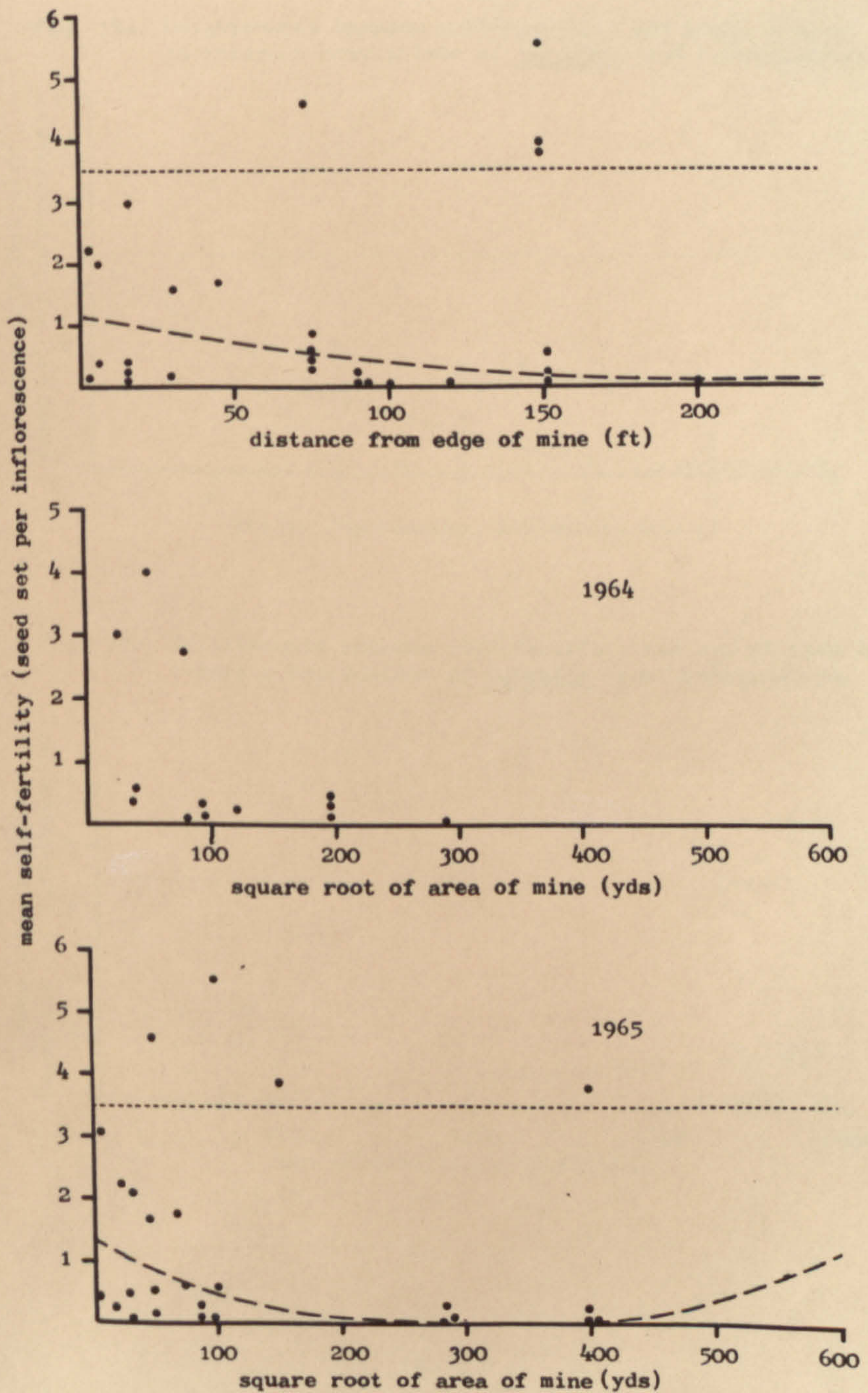
Fig. 33. Relationship between self-fertility and distance from non-tolerant plants in tolerant populations of Agrostis from Cardiganshire. (in this and subsequent set of figures: the points indicate individual populations, points above horizontal line not included in fitted regressions)
