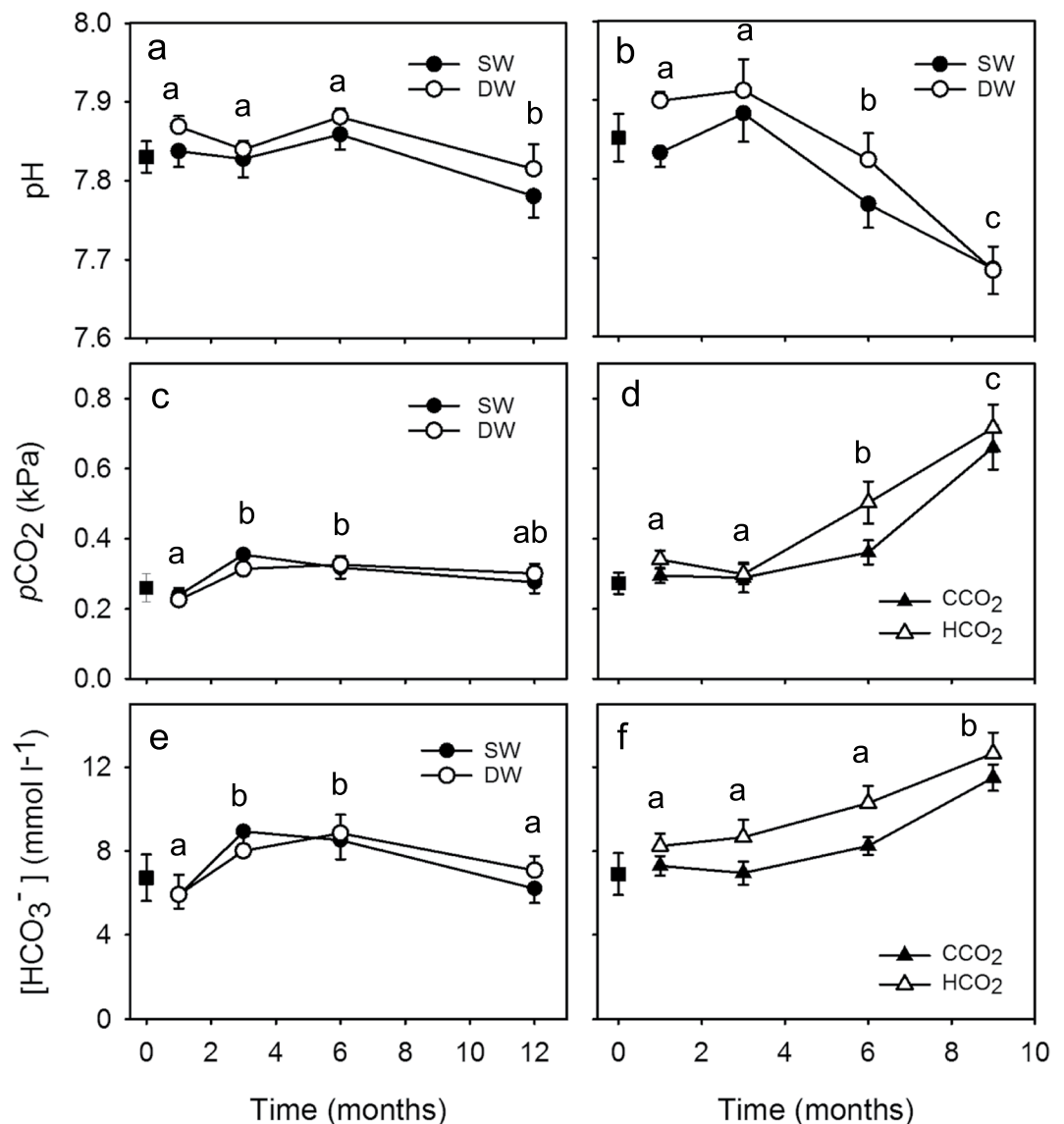
Figure 1. Haemolymph acid-base changes against time in Carcinus maenas : (a) haemolymph pH; (c) partial pressure of \text{CO}_2 ( p\text{CO}_2 ); (e) bicarbonate concentration ( [\text{HCO}_3^-] ). Acid-base changes in Cancer pagurus : (b) haemolymph pH according to salinity and time (SW = full strength seawater, closed circles; DW = dilute seawater, open circles); (d) haemolymph p\text{CO}_2 and (f) haemolymph [\text{HCO}_3^-] according to external p\text{CO}_2 and time (CCO 2 = control, closed triangles; HCO 2 = elevated p\text{CO}_2 , open triangles). Values given as means \pm SEM. For all acid-base variables in Carcinus maenas n = 27, 25, 30 and 24 at 1, 3, 6 and 12 months, respectively. For haemolymph pH in Cancer pagurus : n = 15 at 1 month and n = 16 at 3, 6 and 12 months in SW and DW, apart from 9 months in DW when n = 12 . For haemolymph p\text{CO}_2 and [\text{HCO}_3^-] in Cancer pagurus : n = 15 at 1, 3 and 9 months at CCO 2 and HCO 2 , apart from 9 months in HCO 2 when n = 13 , and n = 16 at 6 months in both conditions. Values with different letters show significant differences (SNK post hoc, P < 0.05 ). In 1a, c and e, both SW and DW shown for reference even though salinity had no effect (significant differences related to changes over time). All values in control crabs at one month (CCO 2 , SW) were similar to those measured in baseline crabs (closed squares; t-tests, \text{df} = 13 , P = 0.457 to 0.996 ).
