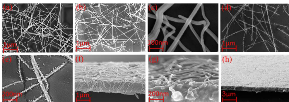
Fig. 2 SEM images of a) AgNWs before embossing, b) after embossing and c) after embossing at higher resolution, d) after embossing and sintered, e) after embossing/sintering at higher resolution. Cross sectional SEM images show f) before embossing, g) before embossing at higher resolution and h) sample that has been embossed and sintered
