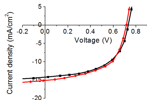
Figure 4: Current-voltage characteristics for PTB7-Th:PCBM OPV using ITO-based electrodes on PET and glass substrates and AgNW-based electrode under 100 \text{ mW/cm}^2 AM1.5 illumination
