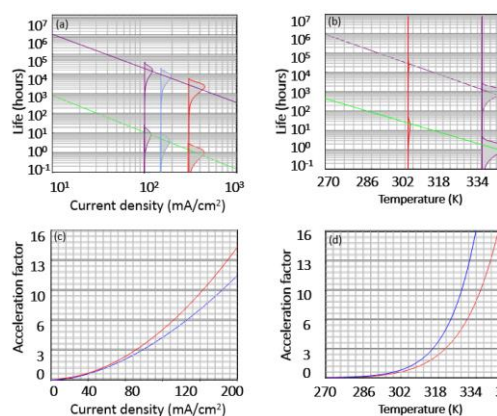
Fig. 5. Regression line fitting for post-processed and 'as-used' AgNW films of the expected time to reach T90% as a function of (a) current density ( \text{mA}/\text{cm}^2 ) and (b) temperature (K). Included in (a) and (b) are the fitted probability distribution functions for each stress level. The Acceleration Factor (AF) as a function of current density and temperature and RH humidity are shown in (c) and (d), respectively
