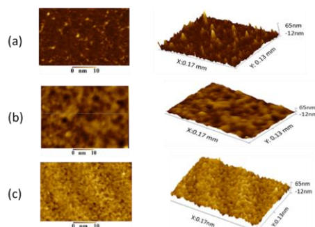
Figure 3: Surface topography images using white light interferometry (WLI), (a) the control sample, (b) post-processed sample and (c) post-processed sample with ZnO overcoating
