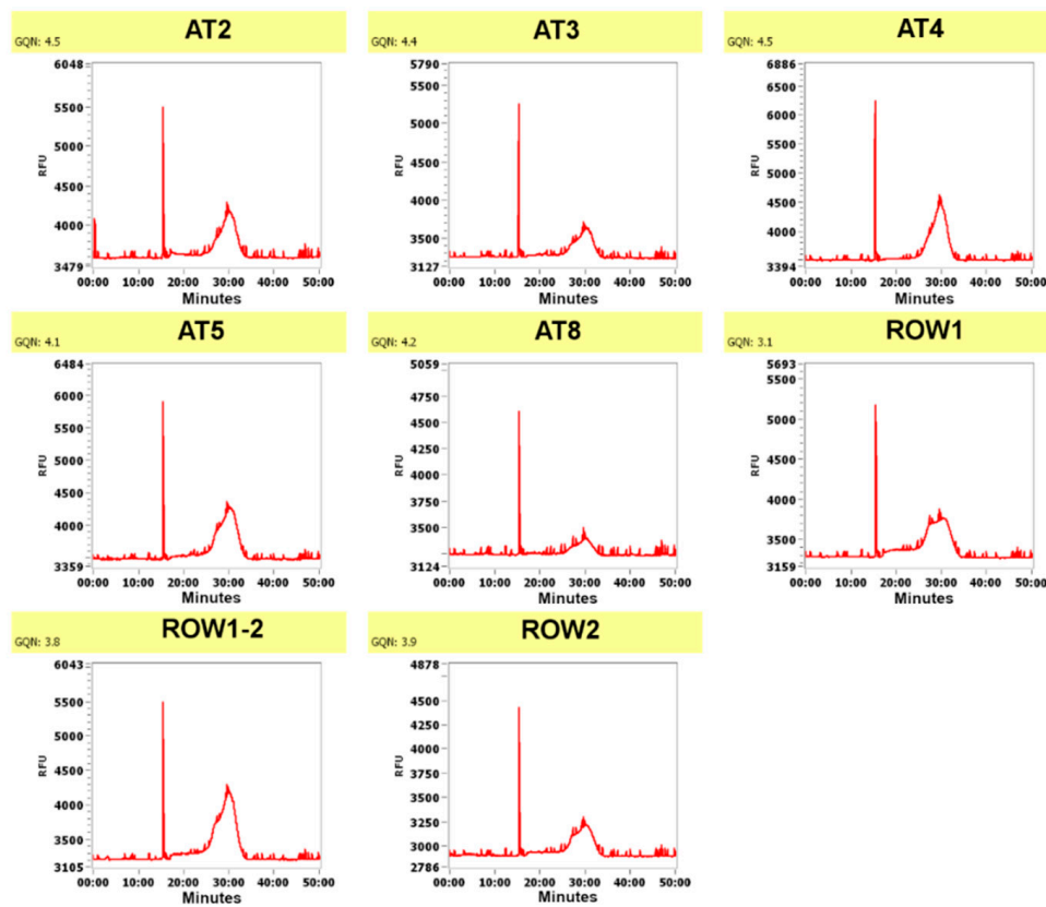
Figure 1. DNA fragment analyzer results for the samples using the PROSize v. 2.0 software. RFU signifies Relative Fluorescence Units (indicating the amount of DNA at a certain size/time), and the X-axis signifies time in minutes as the DNA fragments are separated during capillary electrophoresis.
