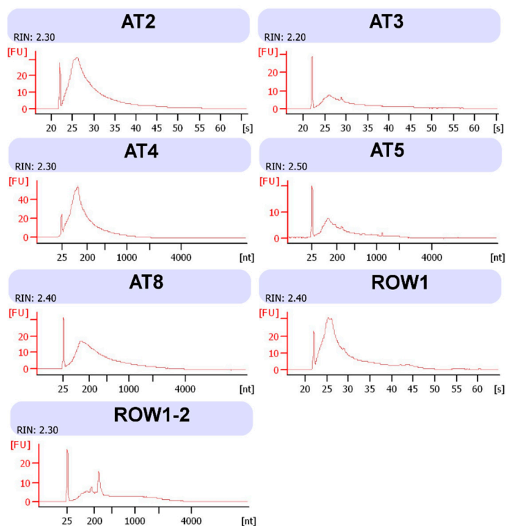
Figure 3. Bioanalyzer Eukaryote total RNA Pico graphs of all RNA extractions in this study. FU indicates Fluorescence Units, [s] indicates seconds and [nt] equals nucleotide size, which is interchangeable to seconds as larger nt fragments take longer to go through the gel.
