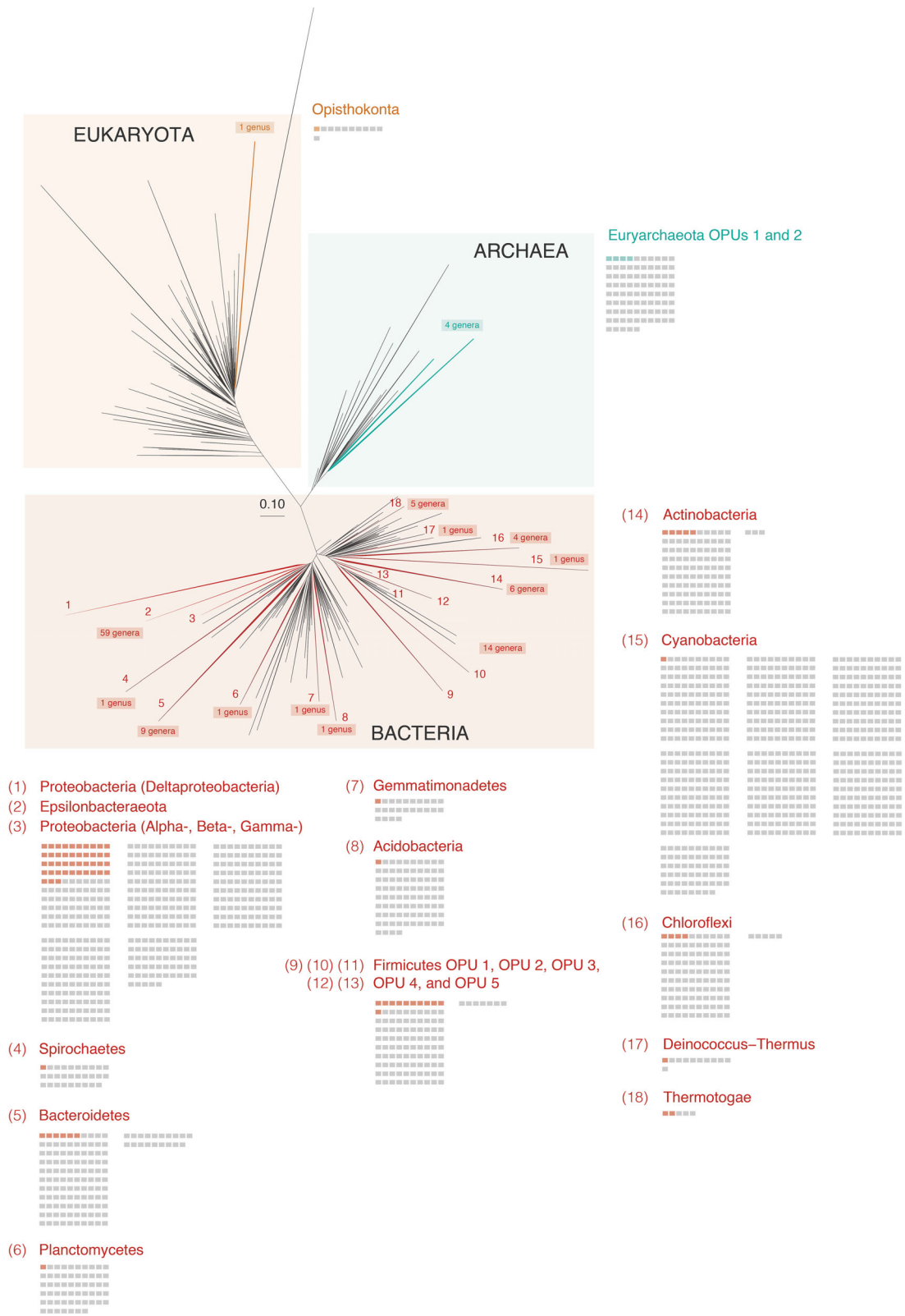
Figure 2. Phylogenetic tree representing the diversity of studied enzymes spanning the three domains of life. The database used for the reconstruction corresponds to the release number 132 from the non-redundant SILVA database for the small sub-unit of the ribosomal RNA (September 2018). Phyla (or corresponding rank for the Eukaryotes) containing the characterised enzymes are depicted in colour (yellow for Eukaryotes, blue for Archaea and red for Bacteria). The graphs represent the families for which enzymes have been characterised (coloured cells) and the total number of families within the phylum according to the SILVA taxonomy (level D4 for taxonomic family). Bigger squares contain 10 \times 10 units to allow easier visualisation. The number of genera with INMARE enzymes indicated for each coloured clade. Scale bar represents substitutions per site. Abbreviations in figure: OPU, Operational Phylogenetic Unit.
