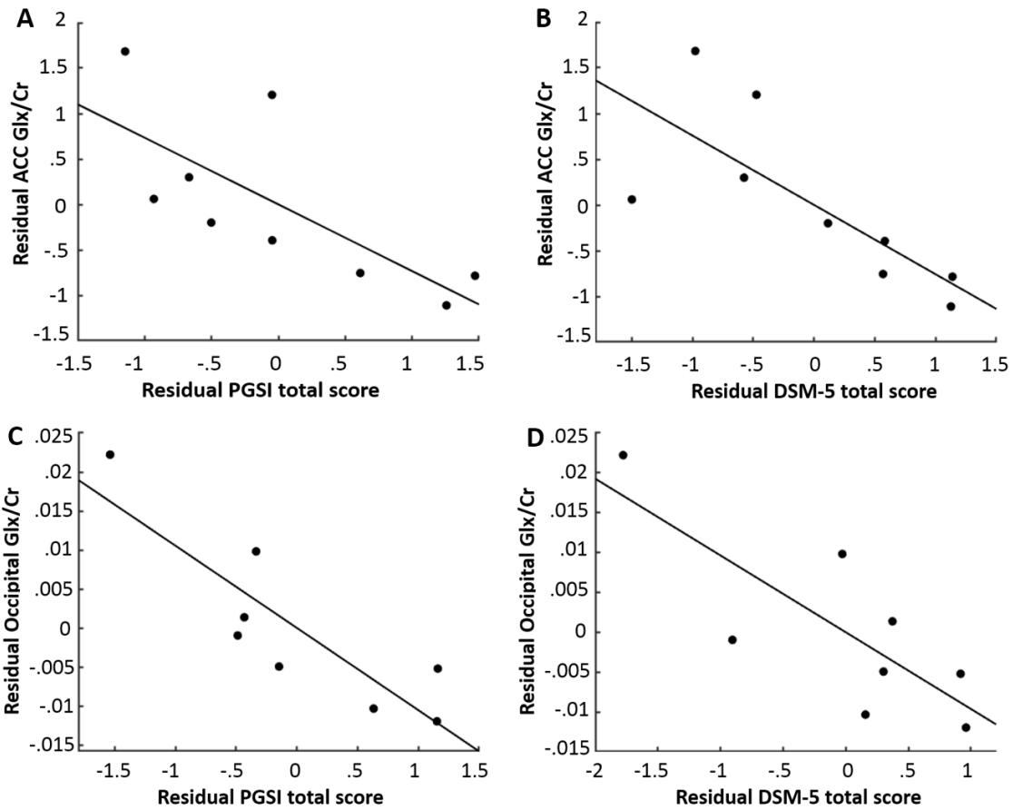
Figure 2. Scatterplots of the significant correlations (adjusted for grey matter content) between MRS variables and gambling severity measures in the GD group only. Scatterplots of the residuals for the correlation between (A) Glx in the ACC and PGSI total scores, (B) Glx in the ACC and DSM-5 total scores, (C) Glx in the occipital voxel and PGSI total scores, and (D) Glx in the occipital voxel and DSM-5 total scores. ACC = anterior cingulate cortex, PGSI = Problem Gambling Severity Index, DSM-5 = Diagnostic and Statistical Manual version 5 – gambling disorder.
