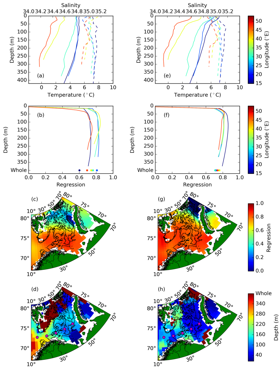
Figure 2. (a) Climatology T – S profiles from EN4 for winter (October to March). Solid line is temperature, and dashed line is salinity. The color shows the location of the profile along the purple dots at 72.5^{\circ}\text{N} shown in (d). The 72.5^{\circ}\text{N} profiles are an example of the transition from AW to BSW. (b) Regression of satellite steric height with EN4 steric height between various integration depths and the surface for winter (October to March). The color shows the location of the profile along the purple dots at 72.5^{\circ}\text{N} shown in (d). (c) Regression of satellite steric height with EN4 in situ steric height between optimum integration depth (OID) and the surface for winter. Hatching shows areas with significance <99\% . (d) Spatially varying OID used in (c). The depth “Whole” on axes refers to integration over the whole water column. White, coastal areas show where data are not available. (e)–(h) are the same as (a)–(d) but for summer (April to September). Black lines show the 220 and 300 m isobaths.
