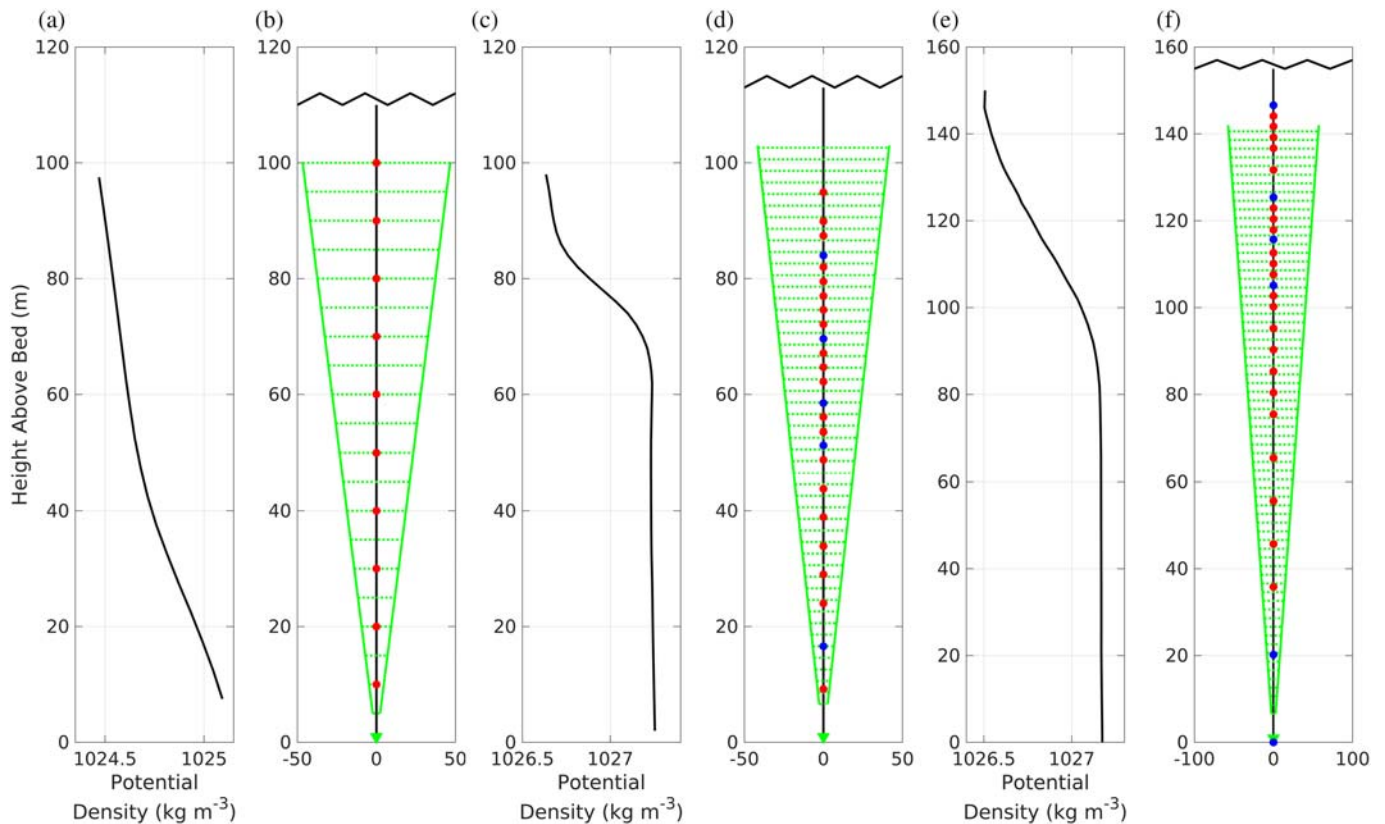
Figure 4. A series of density profiles and mooring diagrams for (a) and (b) the New Zealand (NZ), (c) and (d) the Malin Shelf (SG), and (e) and (f) the Celtic Sea (ST4) moorings. The density profiles (a), (c), and (e) show the average density profile from the moorings. The mooring diagrams (b), (d), and (f) show the ACP data in green with the triangle showing the ADCP position, the solid green lines the spread of the pings, and the dashed lines the boundaries of the ADCP bins. The solid circles show the temperature sensors in red and the temperature and conductivity sensors in blue.
