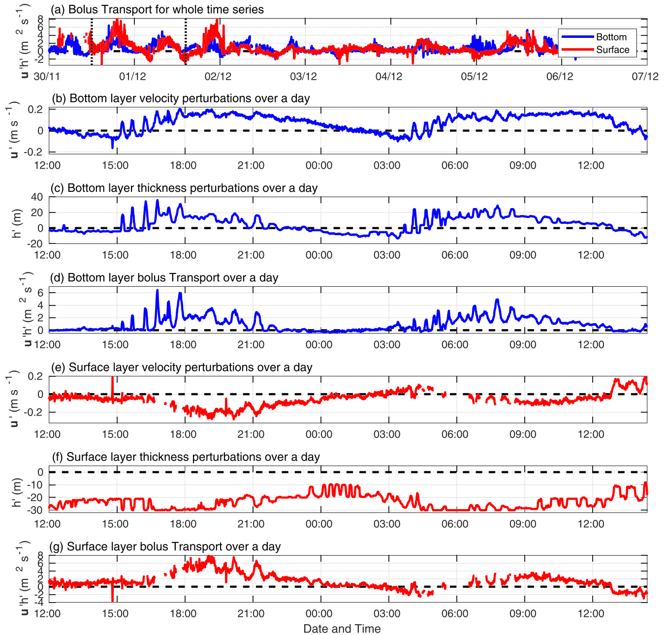
Figure 5. Time series showing the contributions to the bolus transport in the direction of the baroclinic energy flux per unit horizontal length, u'h' ( \text{m}^2 \text{s}^{-1} ) in the surface and bottom layer at the New Zealand mooring: (a) the full time series of instantaneous bolus transport, u'h' , with the selected day shown with vertical dotted lines, (b) the bottom layer velocity perturbations, u' ( \text{m s}^{-1} ) in the direction of the baroclinic energy flux for a selected day, (c) the bottom layer thickness perturbations, h' (m) for a selected day, (d) the bottom layer bolus transport, u'h' , for a selected day, (e) the surface layer velocity perturbations, u' ( \text{m s}^{-1} ) in the direction of the baroclinic energy flux for a selected day, (f) the surface layer thickness perturbations, h' (m) for a selected day, and (g) the surface layer bolus transport, u'h' , for a selected day. The gaps in the surface layer are where the isopycnal was shallower than the most shallow instrument and thus no data were collected for the layer.
