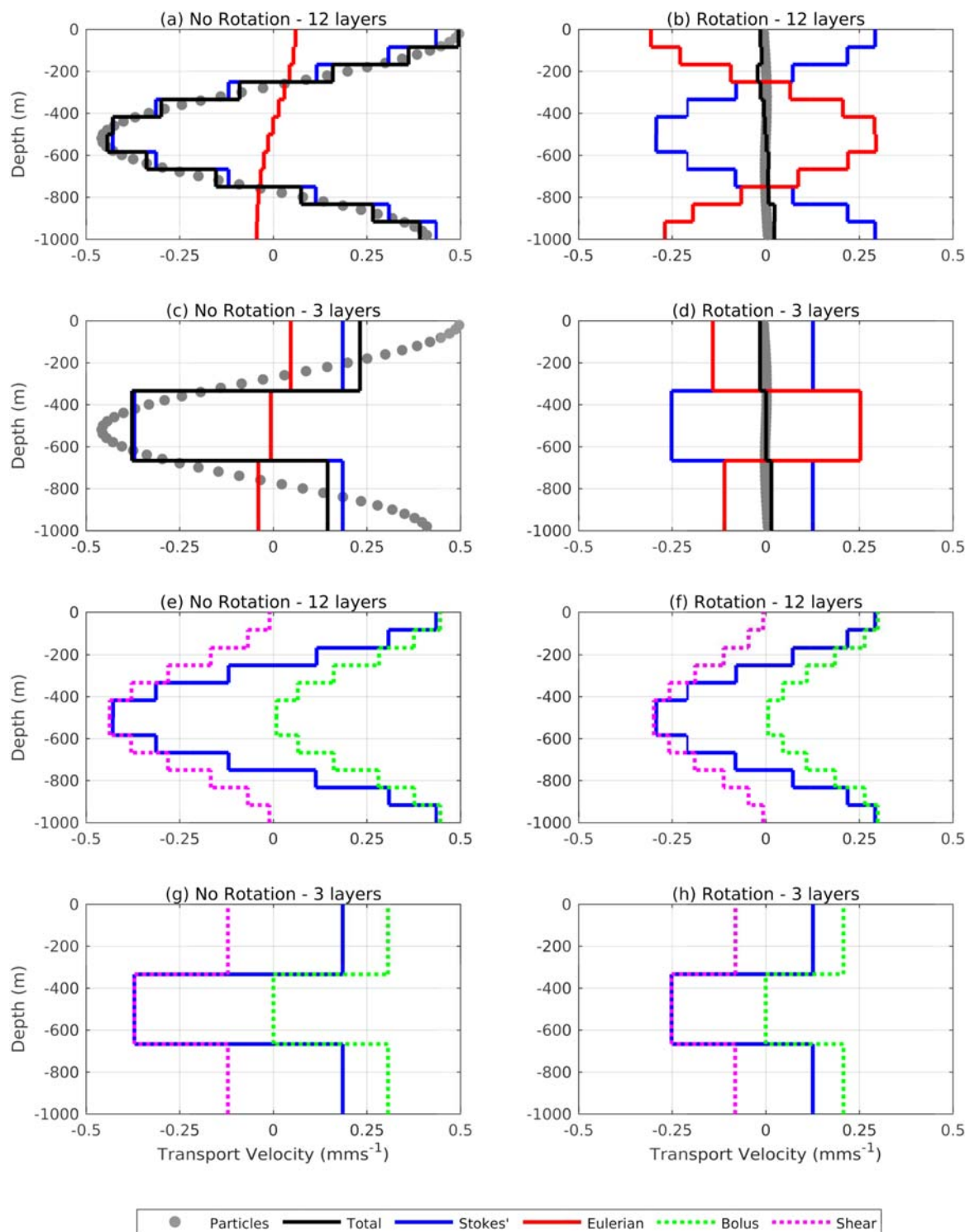
Figure 3. The vertical structure of the transport velocity derived from the particle displacements (gray circles), the total transport (black line), the Stokes' transport (blue line), the Eulerian transport (red line), the bolus contribution to the Stokes' transport (dashed green line), and the shear contribution to the Stokes' transport (dashed magenta line). The transports have been calculated for two different choices for the number of layers: (a, b, e, and f) 12 layers and (c, d, g, and h) three layers, and for both (a, c, e, and g) nonrotating and (b, d, f, and h) rotating cases.
