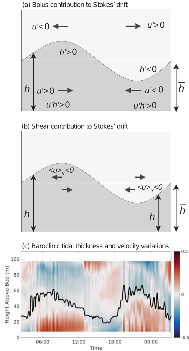
Figure 1. The transport from the Stokes' drift is made up of two contributions (7): (a) the bolus contribution driven by the covariance of layer thickness and the velocity within the layer and (b) the shear contribution from the correlation of the vertical shear in the horizontal velocity and the height of the moving isopycnal. The gray arrows denote the direction of the depth-mean velocity in (a) and the velocity shear in (b). This schematic is comparable to Fig. 4 in Henderson (2016). In (c), the internal tide leads to an onshore bolus contribution from the onshore velocity being correlated with greater layer thickness in the top and bottom layers, illustrated here using observed velocities from a mooring on the New Zealand Shelf.
