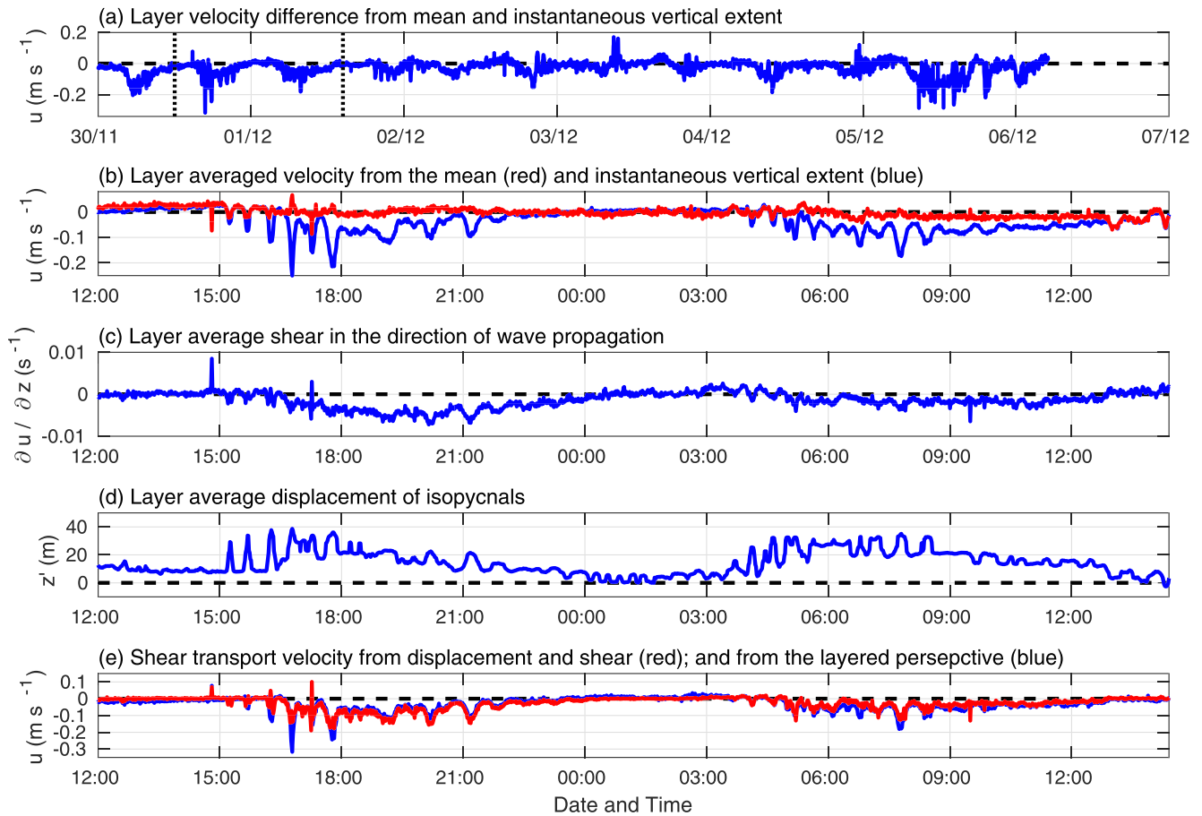
Figure 7. Time series showing the contributions to the shear transport for the middle layer in the direction of the baroclinic energy flux per unit horizontal length for the New Zealand mooring: (a) the difference between the velocity depth averaged over the mean extent of the layer and the instantaneous extent over the whole time series ( \text{m s}^{-1} ), (b) the velocity depth averaged over the mean, red, and instantaneous, blue, extents over a selected day ( \text{m s}^{-1} ), (c) the average shear in the middle layer ( \text{s}^{-1} ), (d) the average displacement of isopycnals in the middle layer (m), and (e) the implied shear transport given by the product of the shear and isopycnal displacement in red and the difference between the velocity depth averaged over the mean extent of the layer and the instantaneous extent.
