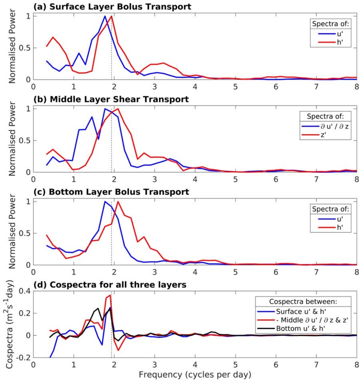
Figure 6. Power spectra and cospectra of the leading contributions to the Stokes' transport for each layer. Each power spectra is normalized by its maximum value. The bolus transport is shown for the (a) surface and (c) bottom layer with the blue line showing the velocity perturbations and the red line showing the thickness perturbations. The shear transport is shown for (b) the middle layer with the blue line showing the layer-averaged shear and the red line showing the layer-averaged displacement. The cospectra are shown (d) between the thickness and velocity perturbations for the surface (blue line) and bottom (black line) layers and the layer-averaged shear and vertical displacement, scaled by the average layer thickness, for the middle layer (red line). The sign of the middle layer cospectra is reversed. The vertical dashed line is the M_2 tidal period.
