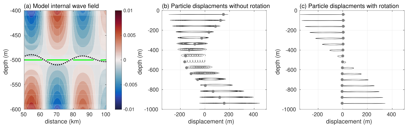
Figure 2. (a) Model subsection of mode 1, internal tide with undulations in temperature surfaces (black), the zero crossing of velocity (green) and zonal velocity ( \text{m s}^{-1} ) in an idealized two-dimensional model with constant N^2 , and model illustration of Lagrangian particle displacements over eight wave periods (with final positions marked by gray circles) from the model (b) without rotation and (c) with rotation.
