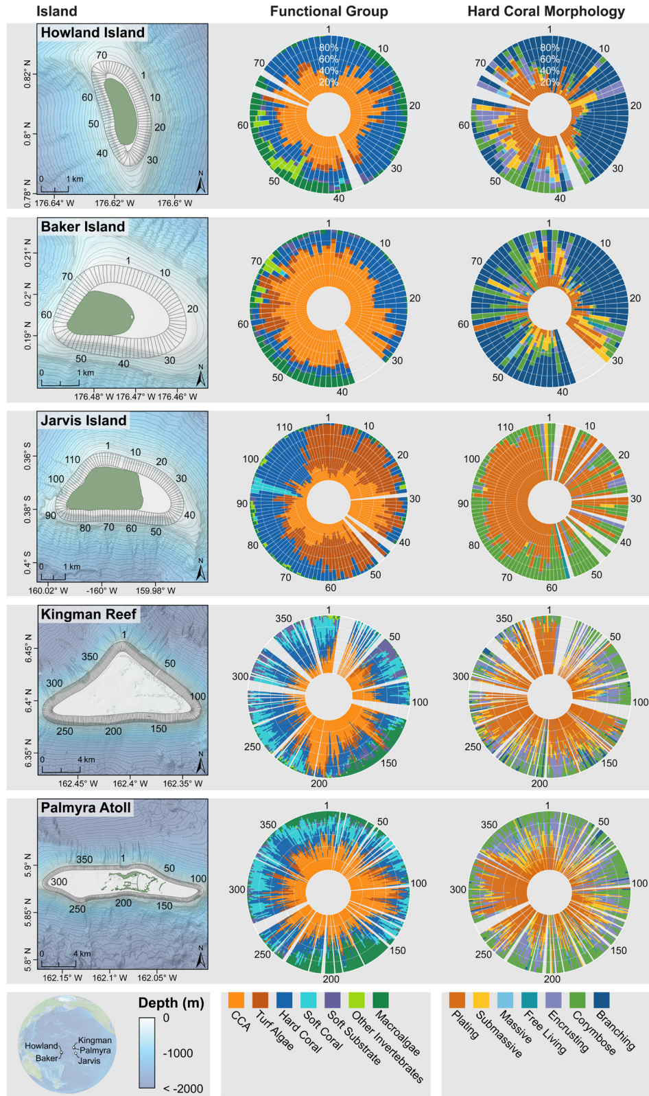
Figure 1. Spatial variations in percentage cover of coral reef benthic functional groups and dominant hard coral morphologies on the outer reef slopes (~15 m depth) of five uninhabited central Pacific islands collected via towed-diver digital image surveys in 2008 across ~140 linear km of reef ( n=6022 images). The white cells around each island are 100-m grid cells that overlap the towed-diver tracks and are used to spatially reference benthic images (their numbers start due north and correspond with those on the island rosette plots). Grey regions on the rosette plots represent missing data regions. The islands are ordered in increasing size top to bottom.
