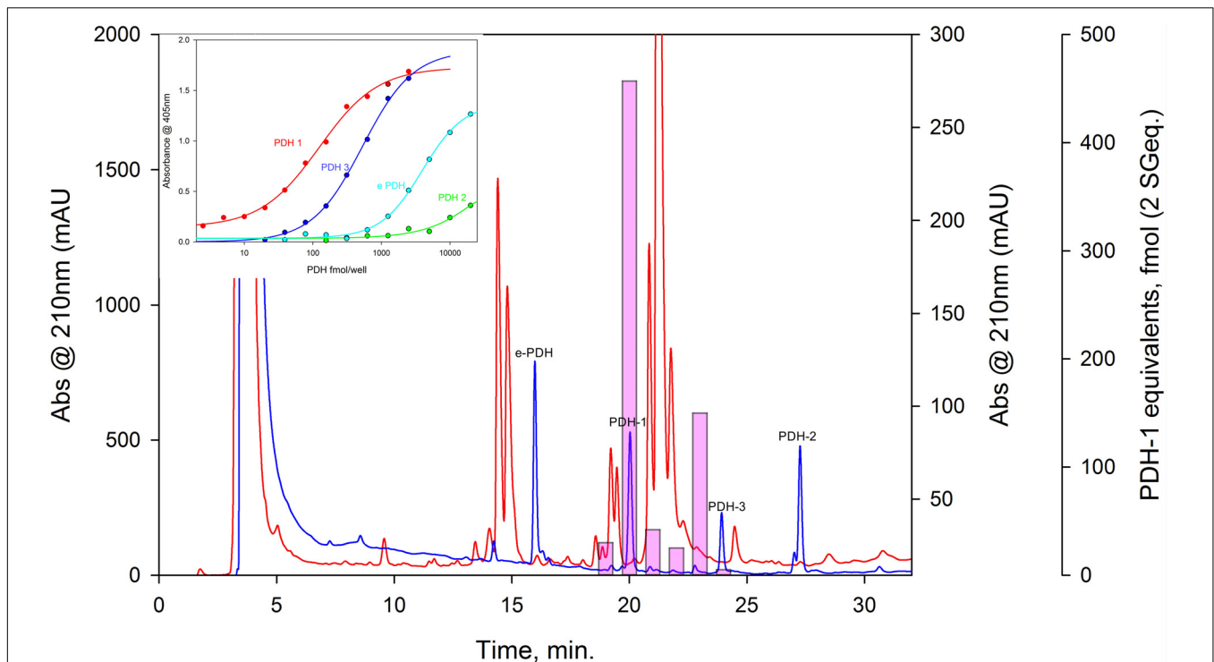
FIGURE 7 | HPLC-EIA of C. maenas SG extracts and standard PDHs. Chromatographic conditions and EIA as described in the text. Red chromatogram shows separation of 50 SG on a Phenomenex C18 column. 1 min. fractions were assayed in duplicate for PDH immunoreactivity, shown as pink bars (PDH-1, 0.5 SG eq. per well, other PDH's, 2.5 SG eq. per well showed no immunoreactivity). Blue chromatogram shows elution profiles of 875 pmol of each PDH, chromatographed immediately after the SG separation. Cross-reactivities of PDH's to the PDH antiserum used (R171) are shown in the insert.
