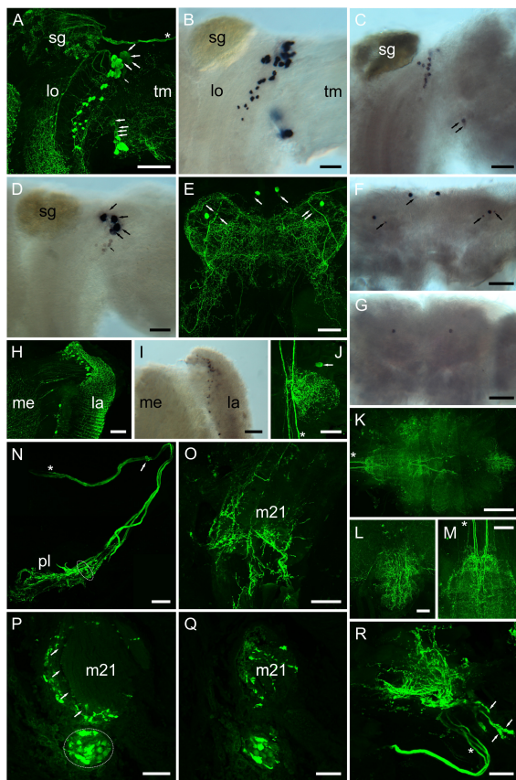
FIGURE 8 | Distribution of PDHs in the central nervous system of C. maenas , detected by confocal ICC ( A, E, H, J–R ) or mRNA by ISH ( B–D, F, G, I ). ( A ) Whole mount image of region between the lobula (lo) and terminal medulla (tm) of eyestalk showing intense labeling of many (ca. 45) PDH IR neurones and fibers. Large arrows highlight four large (40–60 \mu\text{m} ) weakly labeled perikarya in a dorsal position adjacent to the sinus gland, and ventrally four small (ca. 25 \mu\text{m} ) weakly labeled perikarya. Small arrow highlights a number of faintly labeled cells. Asterisk shows position of three prominent axon profiles that exit the eyestalk adjacent to the optic nerve. These profiles are also shown in ( N, R ). ( B ) Whole mount ISH showing hybridization of PDH-1 antisense RNA to many of the profiles shown in ( A ). ( C ) Hybridization of PDH-2 antisense probe to thirteen perikarya adjacent to the sinus gland, and two perikarya on the ventral margin of the terminal medulla (arrows). ( D ) Hybridization of PDH-3 antisense probe to four perikarya (large arrows), corresponding to the weakly labeled cells seen in ( A ). Several (ca. 7) small cell bodies (small arrows) exhibit very weak hybridization signals. ( E ) Whole mount ICC image of the cerebral ganglion. Two pairs of intensely labeled median and lateral perikarya (ca. 40 \mu\text{m} ) and weakly labeled small (ca. 15 \mu\text{m} ) perikarya (arrows) are shown. ( F ) PDH-1 ISH of cerebral ganglion shows correspondence of mRNA labeling with ICC. Arrows indicate small, generally weakly hybridizing perikarya. ( G ) e-PDH ISH of cerebral ganglion showing a single pair of median perikarya. ( H ) Whole mount of lamina showing numerous small (ca. 10–12 \mu\text{m} ) perikarya and fibers. ( I ) PDH-1 ISH showing hybridization signals corresponding to neuronal profiles seen in ( H ). ( J ) Whole mount ICC image of commissural ganglion. Only one neuron was labeled (arrow). Asterisk indicates five descending axon profiles also indicated in ( K, M ). ( K ). Wholemount tiled array (5 \times 4) confocal image of PDH immunopositive structures in the ventral ganglion. ( L–M ) Images of abdominal and subesophageal ganglion taken from ( K ) showing complex patterns of dendrites in both ganglia arising from thick descending axons of interneurons [asterisks in ( K, M )] from within circum-esophageal connectives.
