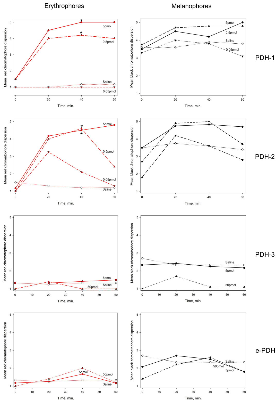
FIGURE 9 | The effect of PDHs on pigment migration in epidermal chromatophores of the 5th walking leg dactylus of C. maenas . Left panel: erythrochromes, right panel: melanophores. Peptides were injected at 0.05–5 pmol per crab for PDH-1, -2, 5–50 pmol per crab for PDH-3, e-PDH, in 10 \mu l volumes. Mean ( n = 6 crabs) chromatophore indices (Hogben-Slome) are indicated. Asterisks indicate significant differences in chromatophore stage ( p < 0.05 , Wilcoxon sign-rank test) 40 min after injection of peptide, compared to 0 min.
