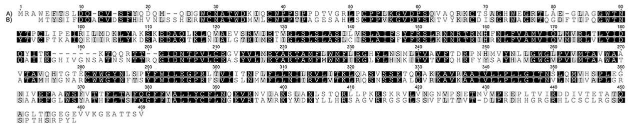
FIGURE 1 | (A) PDHR 41189 and (B) PDHR 43673. Amino acid sequences of two functionally deorphaned PDH receptors. Annotations as referenced in (Oliphant et al., 2018). The six cysteine residues in the N-terminal extracellular domain are marked by asterisks, the seven predicted transmembrane regions are shaded in blue. Putative N-glycosylation sites on the extracellular N-terminal domain are indicated by red lines. Lower panel shows sequence comparisons of both receptors, highlighting identical/similar amino acids as boxed black/gray residues. Gaps added to maximize sequence identity.
