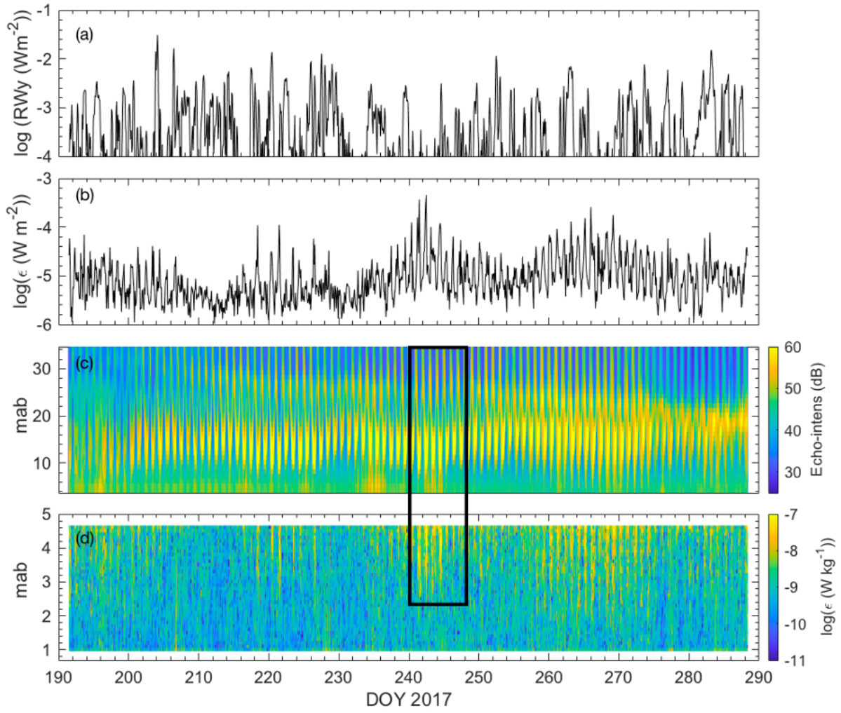
Figure 6. Bottom boundary layer (BBL) dissipation and echo intensity during deployment 4. (a) Rate of energy input at the lake surface RWy ( \text{W m}^{-2} ); (b) Depth integrated, measured dissipation rate, \hat{\epsilon}_{meas}(t) ( \text{W m}^{-2} ), between 0.96 and 4.66 metres above bed (mab); (c) Backscatter intensity, BS (dB) from bottom mounted ADCP covering water column from 3.7 to 36 metres above bed (mab) (d) Vertical structure of the dissipation rate \epsilon(z, t) ( \text{W kg}^{-1} ) in the BBL. Black rectangle shows the 7-day period of the expanded region in Fig. 7.
