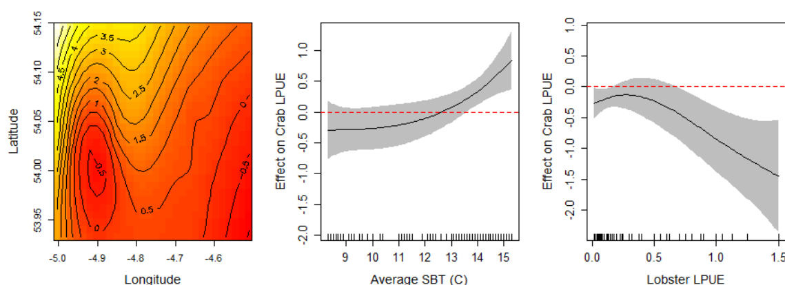
Figure 5.9. Generalised Additive Model (GAM) smoothed term outputs; Crab Model: \text{Crab}_{\text{LPUE}} = s_1(\text{Geolocation}) + s_2(\text{SBT}) + s_3(\text{Lobster LPUE}) + \text{Vessel} .
