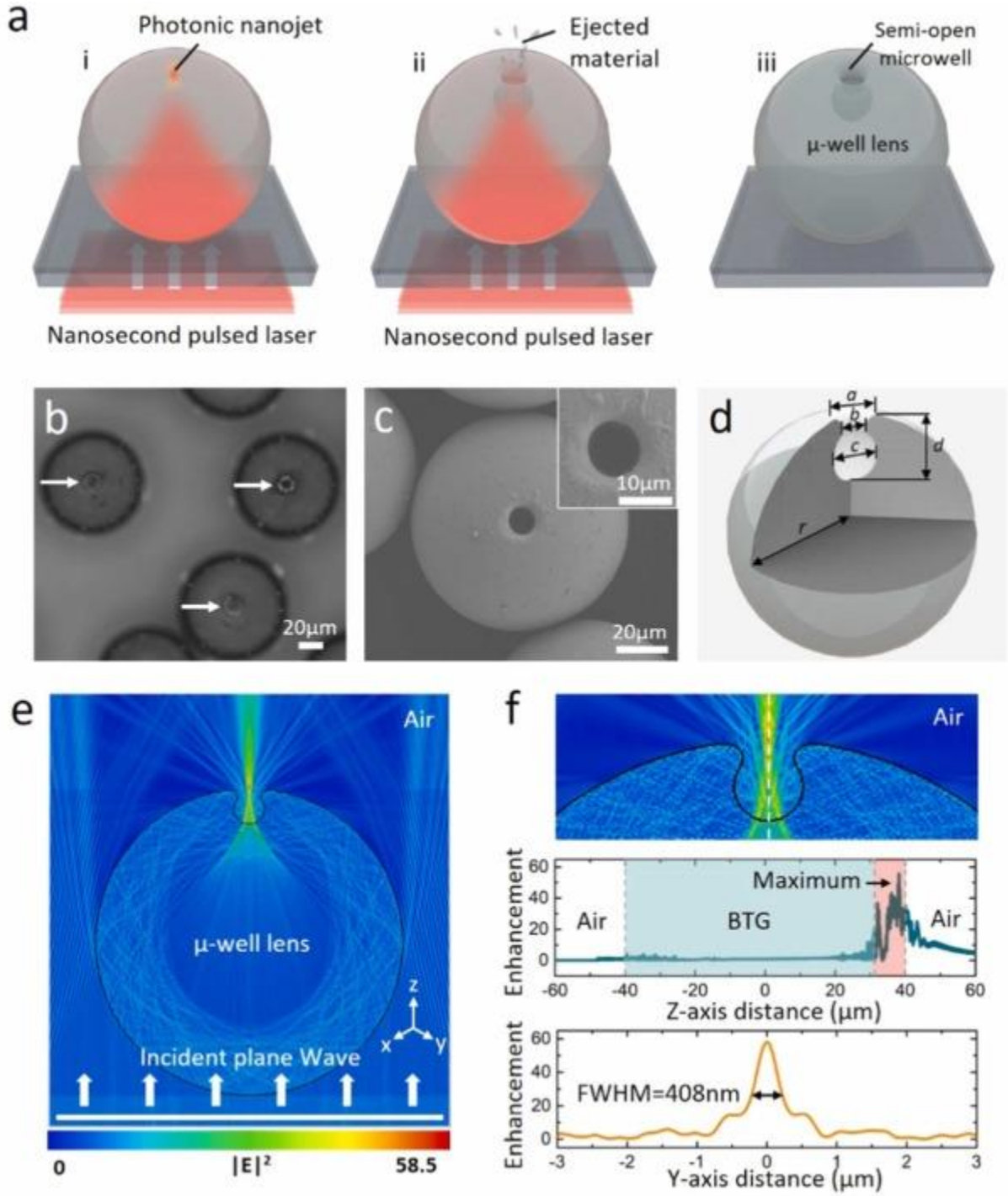
Fig. 1. Fabrication and characterization of the \mu -well lens. (a) Schematic illustration of the fabrication process of the semi-open microwell in the BTG microspheres. (b) Photographic image of the as-prepared BTG microspheres with semi-open microwells. The white arrows indicate the semi-open microwells on each BTG microsphere. (c) Scanning electron microscope (SEM) image of the as-prepared \mu -well lens. (d) Schematic illustration on the dimensions of the fabricated \mu -well lens. (e) Simulation based on finite-difference time-domain showing localized PNJ can be generated inside the semi-open microwell. (f) Plot of the electric field intensity distribution along z-axis and FWHM of the PNJ. The white, green and pink areas in
