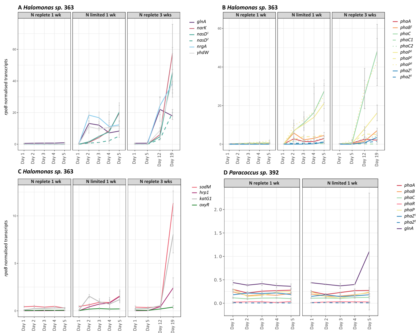
FIG 3 Actively transcribed genes from sea-ice bacterial strains Halomonas sp. 363 and Paracoccus sp. 392 are associated with the nitrogen cycle in Halomonas sp. 363 (A), poly-3-hydroxyalkanoic acid (PHA) production in Halomonas sp. 363 (B), oxygen limitation in Halomonas sp. 363 (C), and PHA production and nitrogen limitation in Paracoccus sp. 392 (D). The sequences were normalized against rpoB , after which the rRNA-associated genes were removed and the relative percentages counted. Note there are different scales on the different graphs. Complete transcriptome annotations against KEGG (release 86, April 2018) (80), PROKKA (1.13) (39), and RAST (2.0) (38) are listed in Tables S3 and S4.
