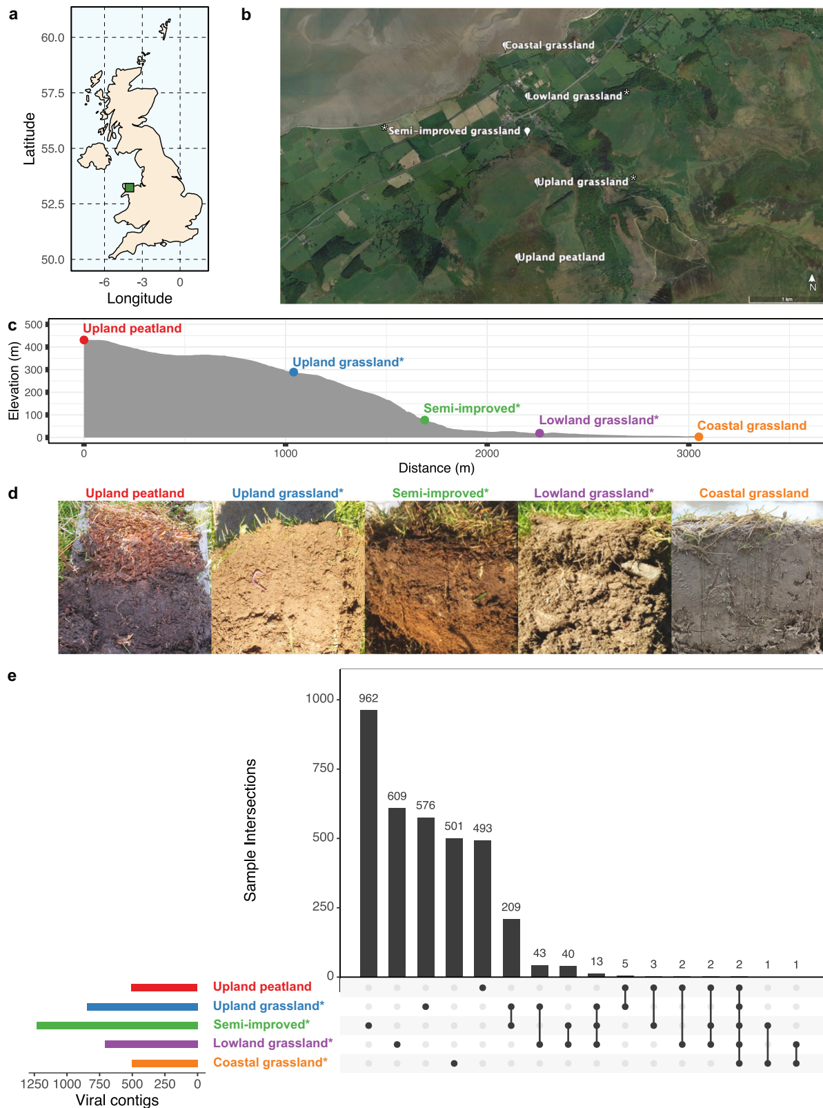
Fig. 1 Soil samples were taken along an altitudinal primary productivity gradient in North Wales, UK ( a ). Sampling sites included upland peatland, (*) three forms of grassland under different management regimes (unimproved upland, semi-improved and improved lowland grassland) and unmanaged coastal grassland ( b - made using Google Earth Pro). Elevation varied by 400 m along the transect ( c ). Site co-ordinates and soil descriptions can be found in Supplementary Table 1. Images of soils from each site can be seen in ( d ) from left to right: upland peatland, upland grassland, semi-improved grassland, lowland grassland and coastal grassland. An Upset plot of the distribution of identified viral contigs ( e ) demonstrates how whilst the majority of viral contigs are found solely at each site, the managed grassland sites share more viral contigs in common than with the upland peat or coastal grassland sites, with the coastal grassland site being almost completely unique.
