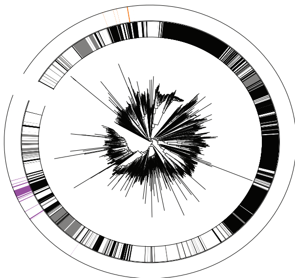
c - Branch 3 ( Kitrinoviricota )
