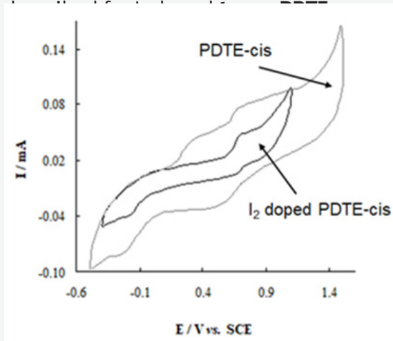
Figure 12 - Cyclic voltammogram of cis -PDTE in monomer free solution (0.1 M TBAPF 6 / MeCN) before and after I 2 doping recorded at \nu = 0.1 V s -1 using a Pt
