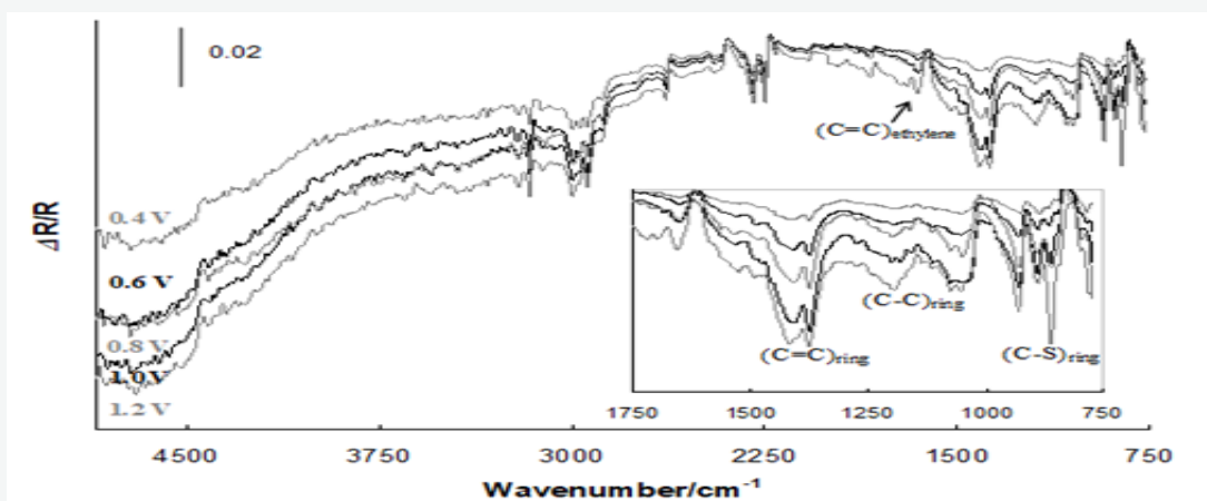
Figure 9 - SNIFTIRS spectra of iodine doped trans-PDTE taken from 0.4 to 1.2 V and expansion of the SNIFTIRS spectra between 1750 and 750 \text{cm}^{-1} . Reference spectra collected at 0 V. Spectra were shifted for clarity.
