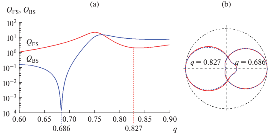
Fig. 9. (Color online) (a) Plots of the functions Q_{FS} (red line) and Q_{BS} (blue line) on a logarithmic scale for a particle with a refractive index n = 4 . (b) The scattering diagrams in the minima of the corresponding functions. The left scattering diagram corresponds to the first Kerker condition (point 1 in Fig. 6), at which backscattering is suppressed completely. The right scattering diagram (point 2 in Fig. 6) corresponds to the second Kerker condition, with minimum forward scattering.
