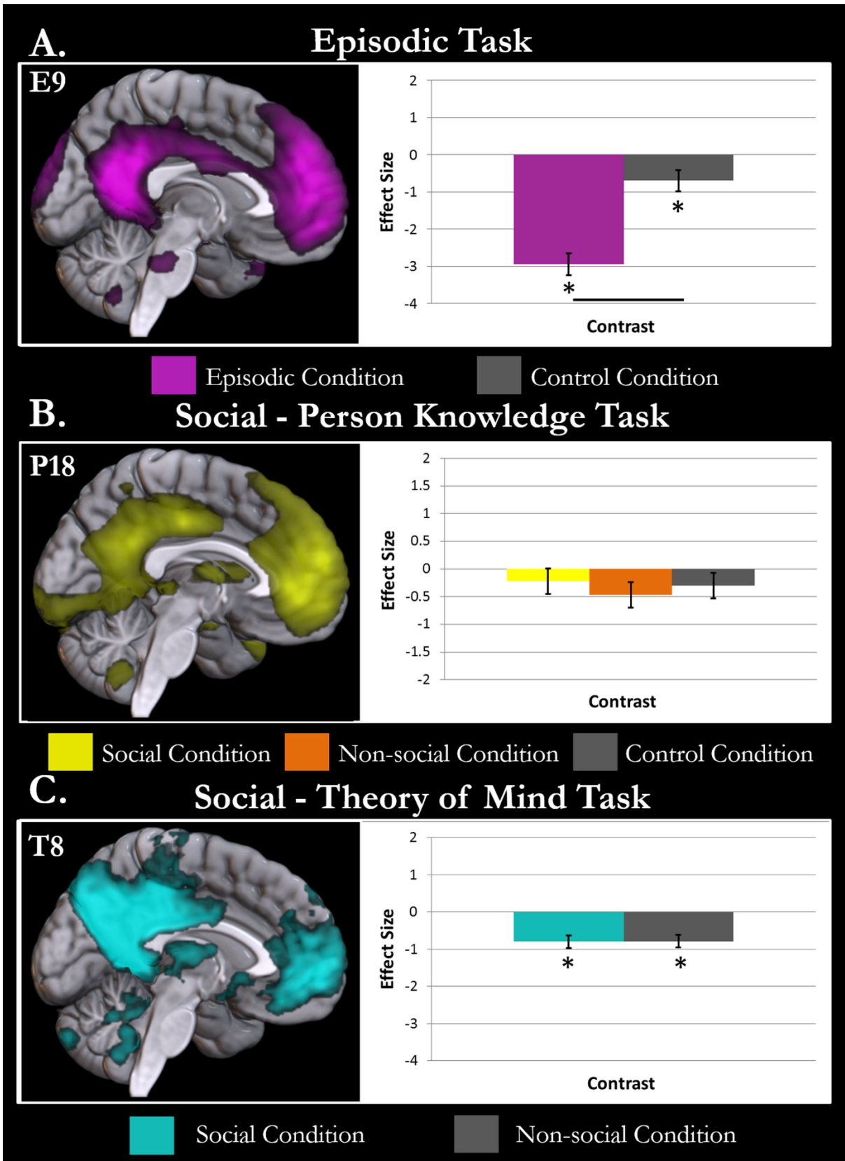
Figure 2. The task relation of the DMN component identified in each task is shown. While only the medial surface is presented here, these components are the same as shown in Figure 1. Conditions with activity significantly different to rest ( p < .05 after Bonferroni adjustment) are highlighted with an asterisk. Differences between conditions are demonstrated by a black line
