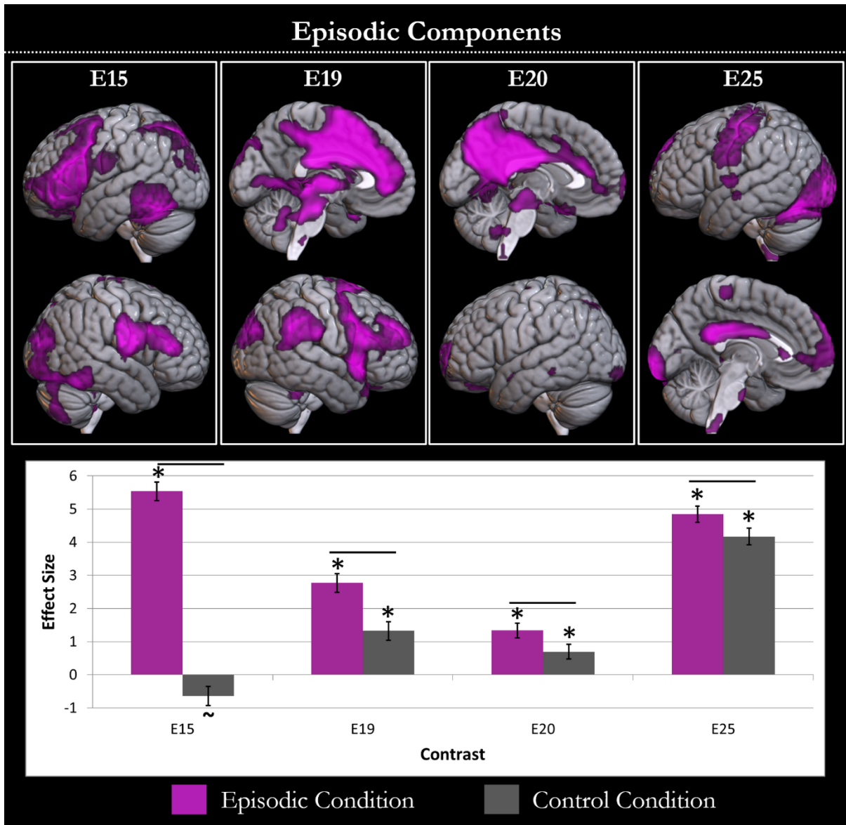
Figure 3. The components with greater involvement in the episodic than the baseline condition are displayed. Each component is shown in violet in the top panel and the task relation of the component is shown in the lower graph. The graph shows the effect size of each component in the episodic (violet) and baseline (grey) conditions compared to rest. Conditions with activity significantly different ( p < .05 after Bonferroni adjustment) to rest are highlighted with an asterisk. A tilde is shown if there is a trend ( p < .1 after Bonferroni adjustment) towards this difference. Differences between conditions are demonstrated by a black line between the condition bars.
