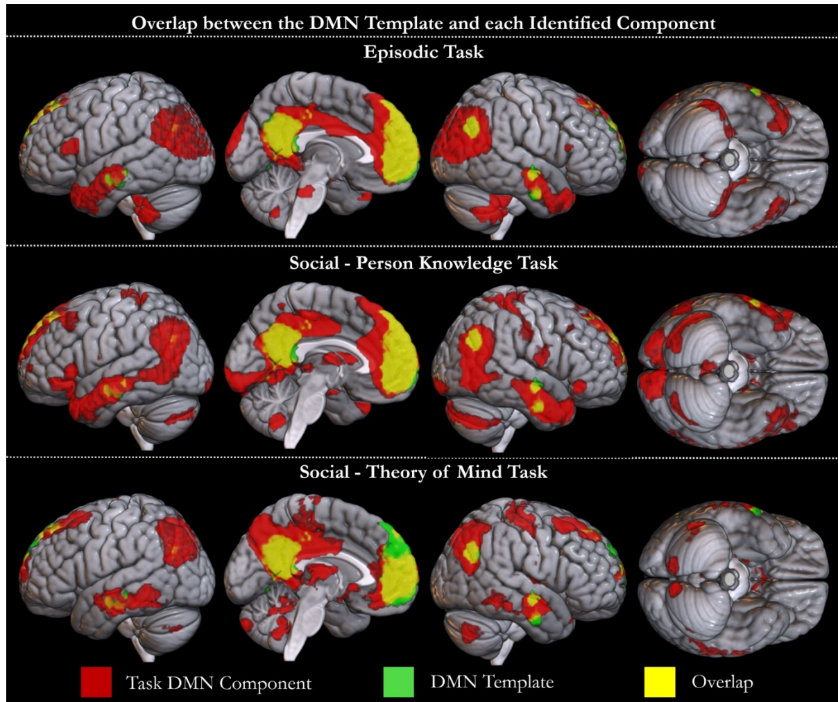
Figure 1. The spatial overlap between the a priori template obtained from Jackson et al., (2019) and the component identified to be the DMN in each task is shown. The components identified in the Episodic Task (E9), Social - Person Knowledge Task (P18) and Social - Theory of Mind Task (T8) datasets are shown in red. The template is shown in green. Overlap is shown in yellow.
