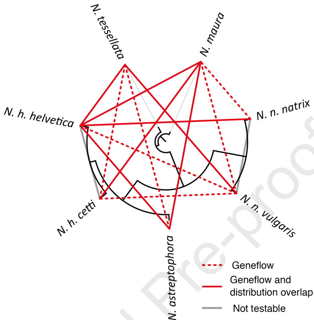
Fig. 4. Results of the HyDe analyses indicating complex and widespread hybridization among Natrix species. Red lines indicate significant evidence for hybridization between the connected taxa. Grey lines indicate species combinations where testing for hybridization was not possible due to the topology. Dotted lines link allopatric taxa; solid lines, sympatric taxa or parapatric taxa with abutting ranges with or without known hybrid zones. The phylogeny is shown as underlying black tree.
