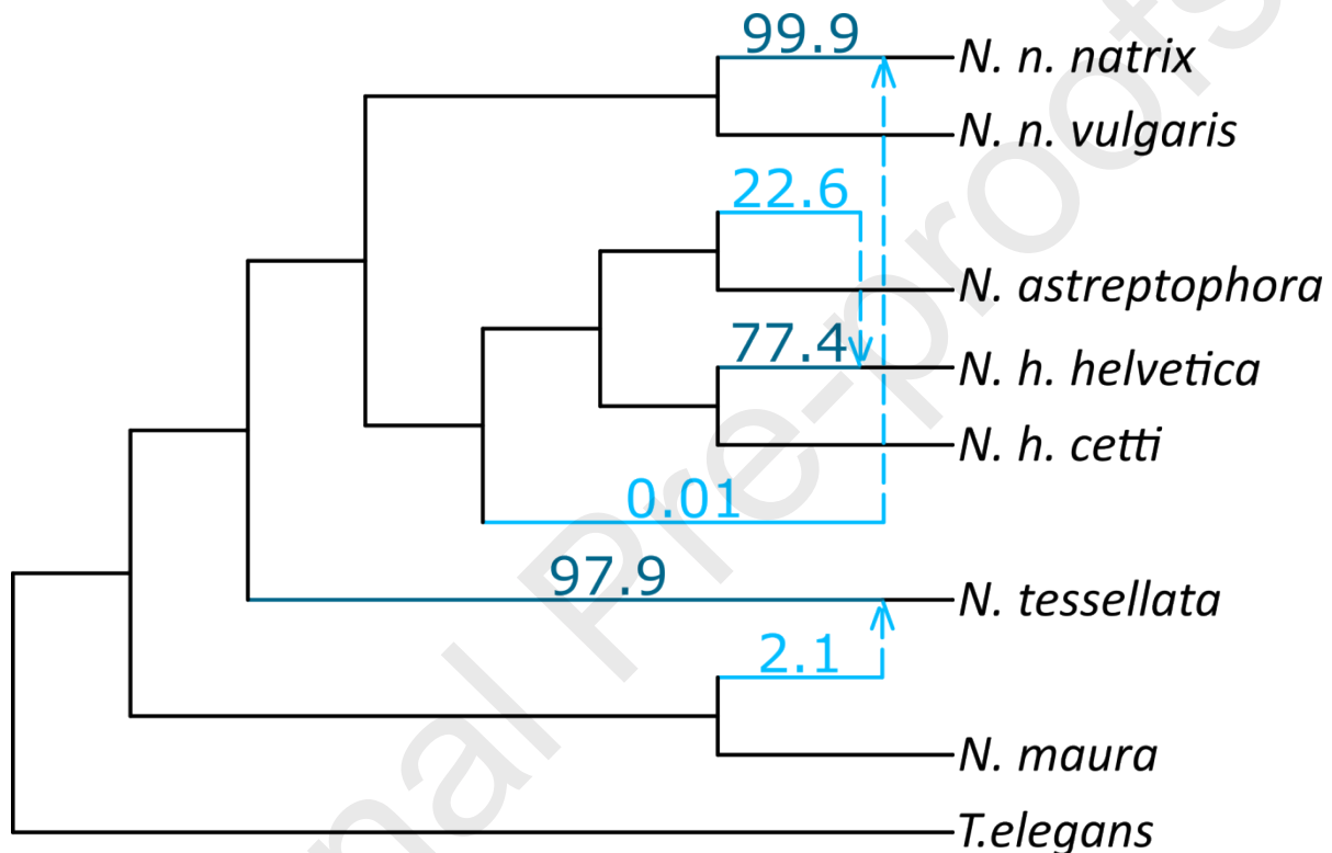
Fig. 3. The best-supported SNAQ result showed three reticulations. Analyses with a higher number of reticulations did not improve the log-likelihood. Reticulations and favored placements are shown in percent. Natrix h. helvetica , for example, was placed in 22.6% of cases as sister to N. astreptophora and in 77.4 % as sister to N. h. cetti .
