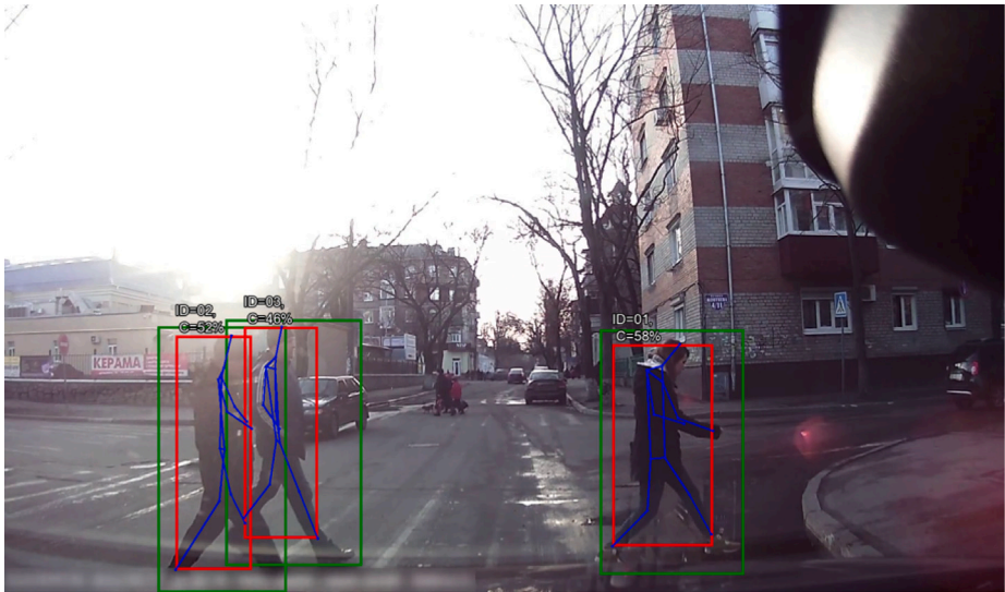
Fig. 3. Multiple pedestrians are being tracked. This is based on the keypoint-generated bounding box (red). The predicted keypoints are connected to create a skeleton for illustration purposes (blue). The ground-truth boxes (green) are for comparison with the generated boxes. The “C” represents the confidence score of the generated bounding box compared to the ground-truth box. The higher the score, the closer the generated bounding box coordinates is to the ground-truth bounding box coordinates (i.e., more accurate). Each tracked pedestrian is given a unique ID to track them along frames.
