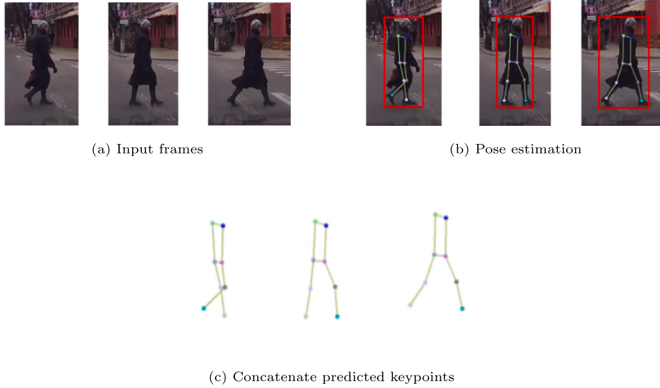
Fig. 2. In this example a pedestrian is crossing the road. Each frame is set 5 frames apart to demonstrate the evolution of the skeleton over time (along frames). In each frame, keypoints are generated from the pose estimator. Using the keypoints, bounding boxes are calculated, allowing to track the pedestrian along the frames. Using the changes of each keypoint, the velocity and direction can be observed to predict the future actions of the pedestrian.
