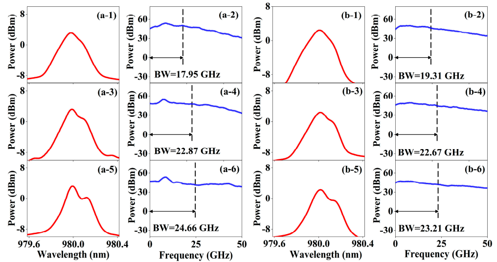
Figure 4. The optical spectra and frequency spectra of the (a-1–a-6) XP mode and (b-1–b-6) YP mode of the VCSEL1. (a-1,a-2) and (b-1,b-2) k_{inj} = 50 \text{ ns}^{-1} and \Delta f = 20 \text{ GHz} ; (a-3,a-4) and (b-3,b-4) k_{inj} = 50 \text{ ns}^{-1} and \Delta f = 30 \text{ GHz} ; (a-5,a-6) and (b-5,b-6) k_{inj} = 50 \text{ ns}^{-1} and \Delta f = 40 \text{ GHz} .
