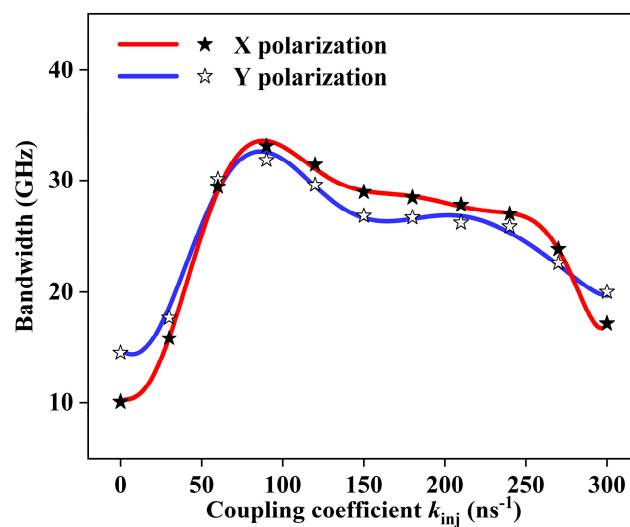
Figure 7. The variation of polarization chaos bandwidth for XP and YP modes of VCSEL1 with the coupling coefficient.
