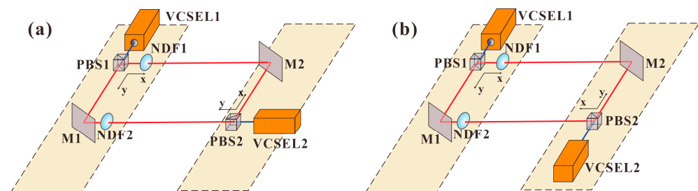
Figure 1. Schematic for polarization chaos in two mutually coupled VCSELs in two scenarios of (a) parallel injection and (b) orthogonal injection. VCSEL1 and VCSEL2, vertical-cavity surface-emitting lasers; PBS1 and PBS2, polarizing beam splitters; NDF1 and NDF2, neutral density filters; M1 and M2, mirrors.
