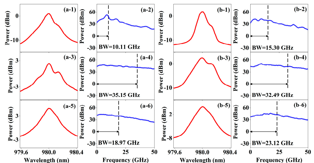
Figure 6. The optical spectra and frequency spectra of the (a-1–a-6) XP mode and (b-1–b-6) YP mode of the VCSEL1. (a-1,a-2) and (b-1,b-2) k_{inj} = 10 \text{ ns}^{-1} and \Delta f = 40 \text{ GHz} ; (a-3,a-4) and (b-3,b-4) k_{inj} = 80 \text{ ns}^{-1} and \Delta f = 40 \text{ GHz} ; (a-5,a-6) and (b-5,b-6) k_{inj} = 300 \text{ ns}^{-1} and \Delta f = 40 \text{ GHz} .
