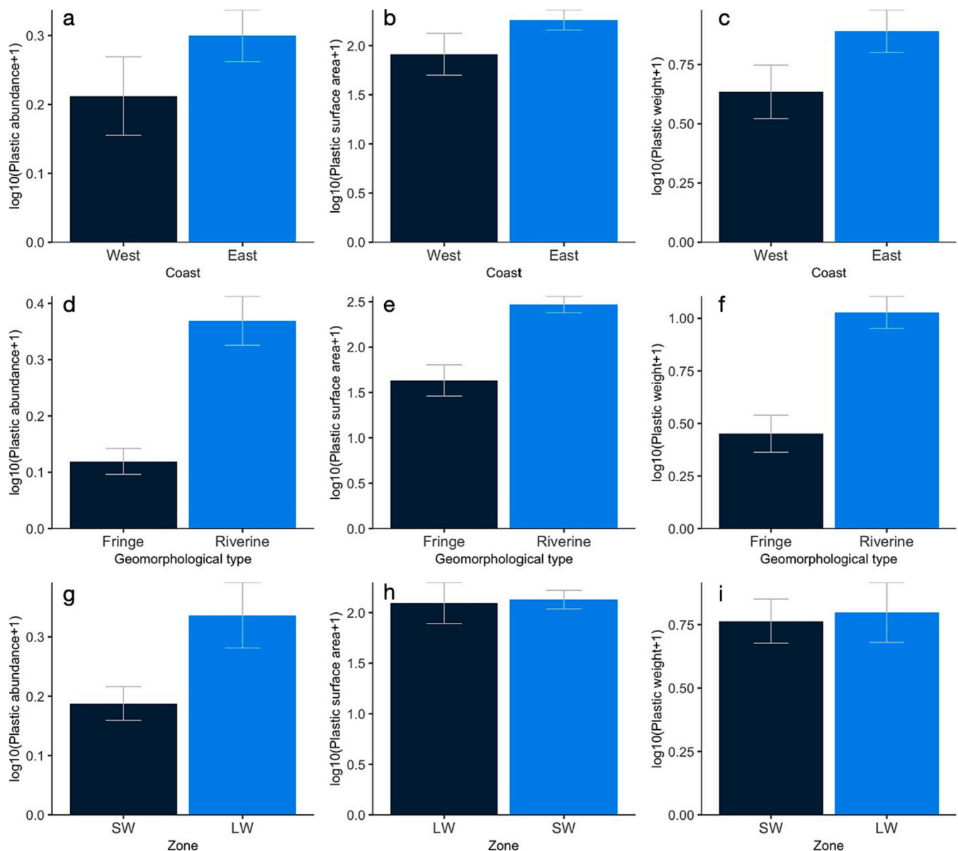
Fig. 4. Effects of coasts, geomorphological type and zones (LW: landward. SW: seaward) on the mean \pm s.e. abundance (items \text{m}^{-2} ), surface area ( \text{cm}^2 \text{m}^{-2} ) and weight ( \text{g m}^{-2} ) of plastic litter in Cebu mangroves.
