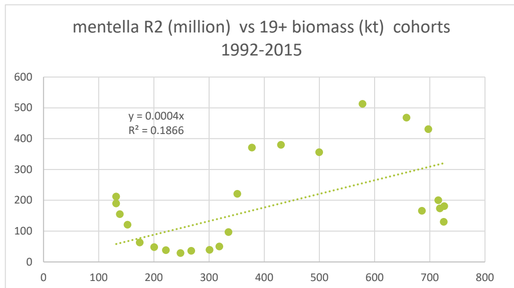
Figure 13. Spawning–stock biomass (SSB) age 19+ (bottom) vs. age 2 recruitment during 1992–2015 as estimated by the last ICES assessment (ICES, 2018a).
