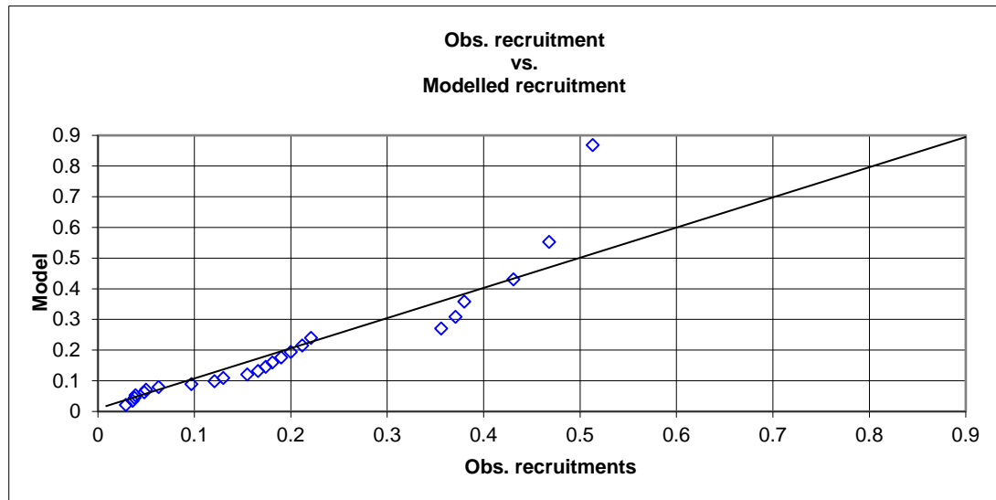
Figure 7. Observed vs. modelled recruitment for stochastic stock–recruitment function.
