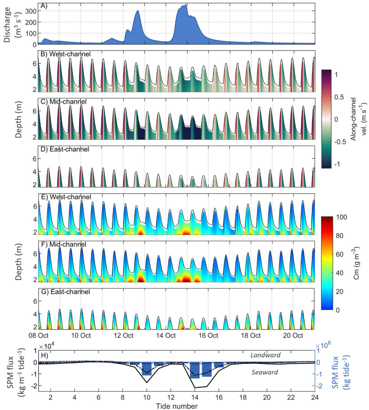
Figure 8: Station 1 (Tal-y-Cafn) during the survey in October 2017: (A) River Conwy discharge ( m^3 s^{-1} ); (B-D) Along-channel velocity ( m s^{-1} ) at the west/mid/east moorings; (E-G) SPM mass concentration
