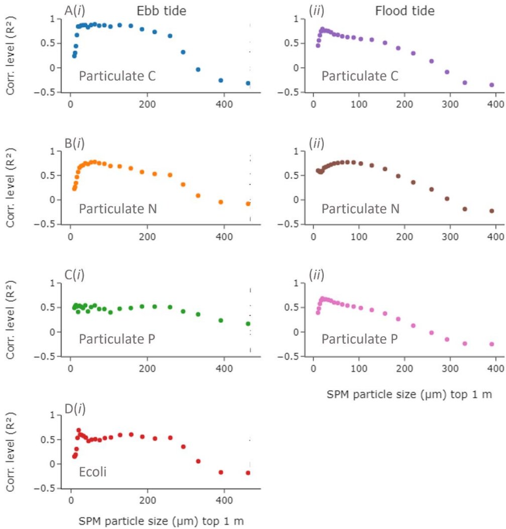
Figure 9: Correlation values ( R^2 ) of gross concentration of the biogeochemical component with individual particle size classes, plotted against particle size for particulate (A) carbon, (B) nitrogen, (C) phosphorus, and (D) FIOs using all samples collected during all sampling campaigns at Station 1 (Tal-y-Cafn). Left panels (i) denote correlations during the ebb tide, and right panels (ii) during the flood tide (there were not enough data for FIO analysis during the flood tide). R^2 values are statistically significant for R^2 > 0.6 .
