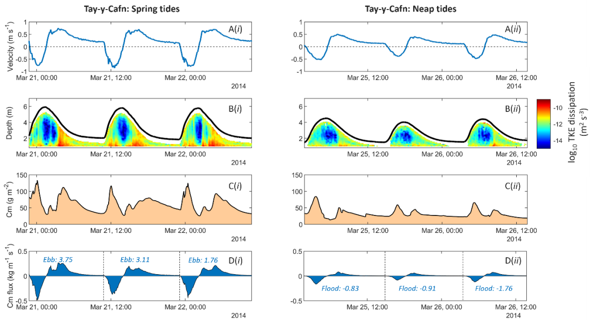
Figure 6 Station 1 (Tal-y-Cafn) during March 2014: (A) Depth-averaged along-channel velocity ( m s^{-1} ); (B) \log_{10} TKE dissipation rate ( m^2 s^{-3} ); (C) depth-integrated SPM mass concentration ( g m^{-2} ); and (D) SPM mass flux ( kg m^{-1} s^{-1} ). The left panels (i) show the data during three spring tidal cycles whereas the right panels (ii) show the data during three neap tidal cycles. In (A) and (D), positive values indicate the ebb tide (up-estuary) direction.
