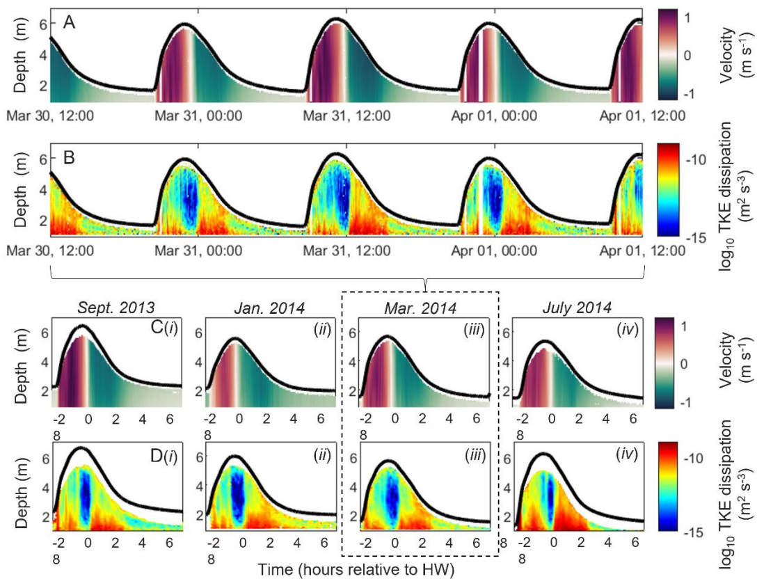
Figure 2: Station 1 (Tal-y-Cafn): ADCP measurements during four successive tidal cycles (March-April 2014), illustrating (A) along-channel velocities ( m s^{-1} , positive values indicate upstream direction during the flood tide), and (B) the corresponding along-channel turbulent kinetic energy (TKE) dissipation rate ( m^2 s^{-3} ) presented on a \log_{10} colour scale. Panels (C) and (D) depict along-channel velocity and \log_{10} TKE dissipation rate, respectively, during the spring tidal cycles in (i) Sept. 2013, (ii) Jan. 2014, (iii) Mar. 2014, and (iv) July 2014. Data in (i-iv) are displayed in phase-averaged form relative to high water (HW), with averages taken over four spring tidal cycles; for instance, the data in A and B have been averaged to produce C(iii) and D(iii), respectively. The black line in all panels indicates the water depths (m).
