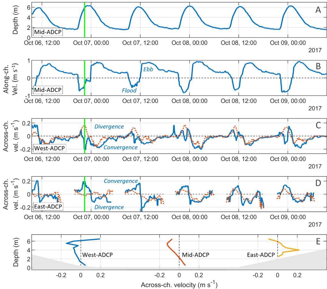
Figure 3: Station 1 (Tal-y-Cafn): Demonstrates the evidence of axial convergence from three ADCP deployments during 06 – 09 October 2017. Panel (A) presents a timeseries of mid-channel water depths, and panel (B) displays timeseries of longitudinally-resolved surface velocities (positive values indicate ebb flow). Timeseries of laterally-resolved surface velocities (blue curves) and bottom velocities (orange dotted curves) are displayed for west- (C) and east-channel (D) ADCP deployments (positive values indicate northwest directed flows). Panel (E) illustrates the instantaneous velocity vectors at each depth bin through a west-east transect at Tal-y-Cafn at 22:25 on October 06 (indicated by the horizontal green line in panels A-D). Positive values indicate southeast directed flows. The pattern shown was consistent throughout the ADCP deployments from October 06 to 20, 2017, except during periods of large river flows (see Supplementary Material, Figs. S2-S3).
