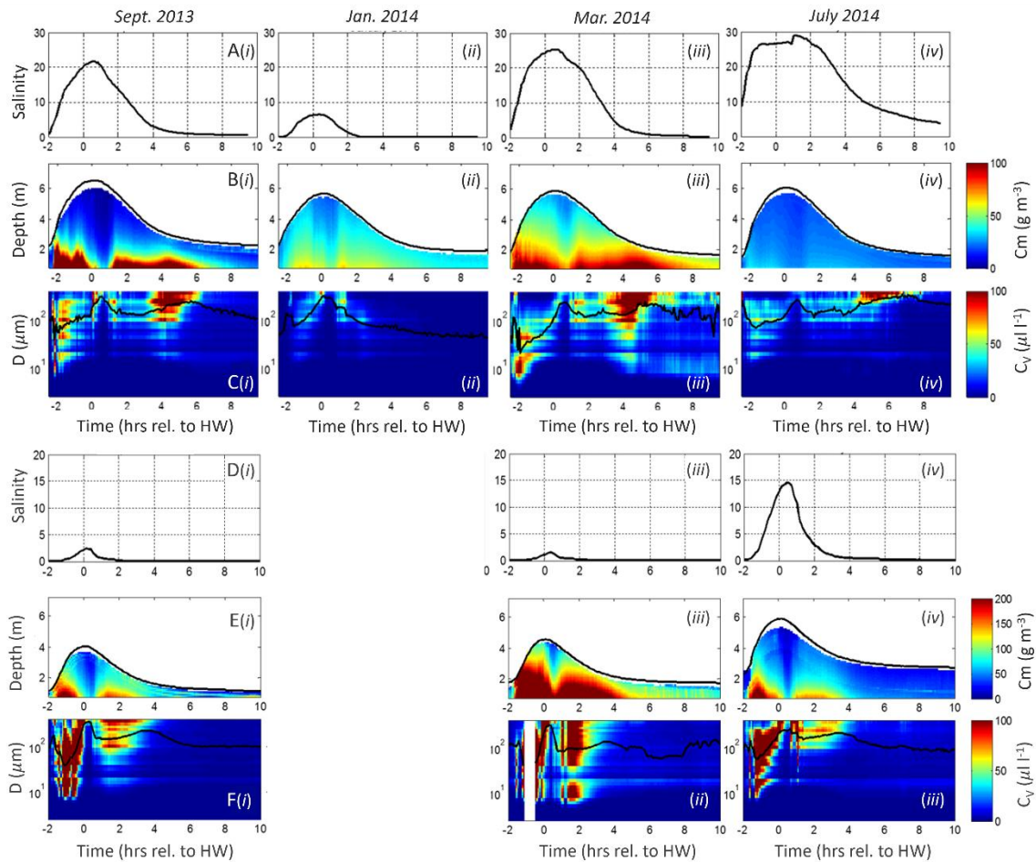
Figure 4: Rows (A-C) display measurements at Station 1 (Tal-y-Cafn), showing (A) salinity, (B) SPM mass concentration ( C_m ), and (C) volume concentrations of particle size spectra ( C_v ), during the four sampling periods: (i) Sept. 2013, (ii) Jan. 2014, (iii) Mar. 2014, and (iv) Jul. 2014. The particle size spectra also present the median particle size D_{50} (black line). The data represent averages taken from four successive spring tides. Corresponding measurements for Station 2 (Dolgarrog) are shown in rows (E-F) during three sampling periods: (i) Sept. 2013, (ii) Mar. 2014, and (iii) Jul. 2014. The data for the Jan. 2014 sampling period was found to be erroneous and is therefore not shown.
