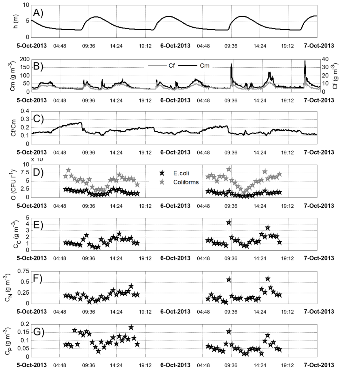
Figure 5: Station 1 (Tal-y-Cafn), presenting data from four consecutive tides in October 2013, including: (A) Water level; (B) Chlorophyll ( C_f ) and SPM mass concentration ( C_m ); (C) Chlorophyll/SPM mass concentration ratio; (D) Particulate concentrations of faecal indicator organisms (FIOs) for E. coli and Coliforms; (E) Particulate carbon concentration ( C_C ); (F) Particulate nitrogen concentration ( C_N ); and (G) Particulate phosphorus concentration ( C_P ).
