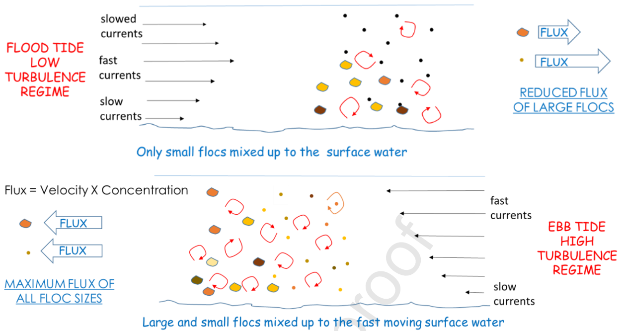
Graphical abstract: (upper panel) Suppression of turbulence reduces SPM flux on the flood tide at Tal-y-Cafn. (lower panel) Normal development of turbulence maintains SPM flux on the ebb tide at Tal-y-Cafn.
