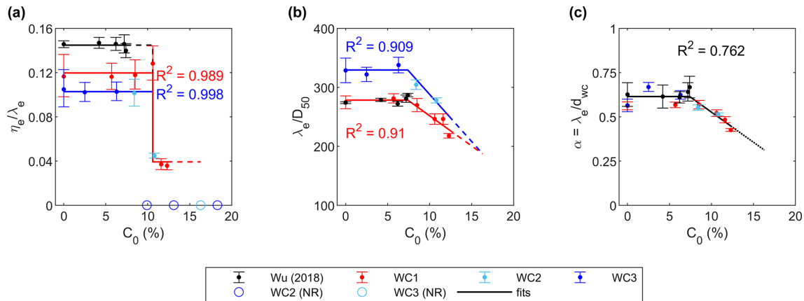
Figure 6. Equilibrium ripple steepness, RS = \eta_e/\lambda_e , (a) ; non-dimensional ripple wavelength, \lambda_e/D_{50} , (b) ; and the \alpha parameter, \alpha = \lambda_e/d_{wc} , (c) , as a function of initial bed clay content, C_0 , for Wu et al. (2018) and WC1–WC3. Open circles show that no ripples (NR) were present and dots are based on measured values of \eta_e , \lambda_e , and \alpha and their error bars. Solid lines correspond to least-squares fits to the data with R^2 values quoted.
