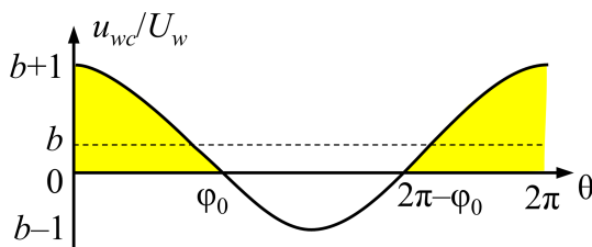
Figure B1. Plot of Eq. (B1), where shaded area represents d_{wc} in Eq. (B3).
