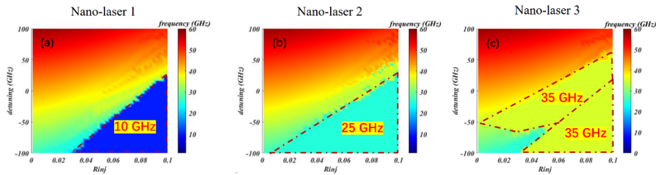
Fig. 11. Distribution of the oscillation frequency of nano-lasers in the third scenario of the nano-laser array with optical injection shown in Fig. 1(c) when \alpha=2 and the coupling rate k_{12} = k_{23} = 5 \times 10^9 . The modulation frequency of the three master lasers are set to be 10 GHz, 25 GHz and 35 GHz respectively for nano-laser 1-3. The modulation depth of the three master lasers are set to be 0.3.
