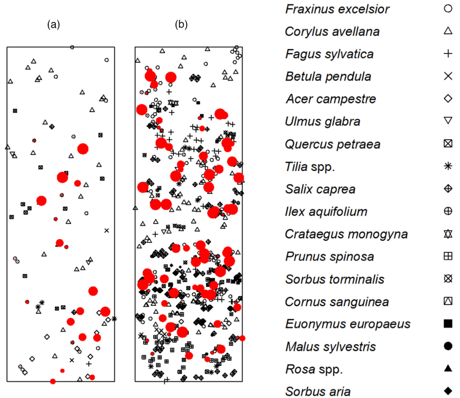
FIGURE 2 Locations and species of all trees in two transect subplots (19.8 m × 121.9 m) generated using the 'spatstat' R package showing the prevalence of ADB. (a) is an example of one of the 'old growth' subplots in transect 1. (b) is one of the 'young growth' subplots in transect 3. The red dots are infected Fraxinus excelsior trees, with their size representing the severity of infection. Asymptomatic F. excelsior trees are shown as open circles. The data illustrated in these spatial plots were used to calculate species mingling, size dominance and tree density.
