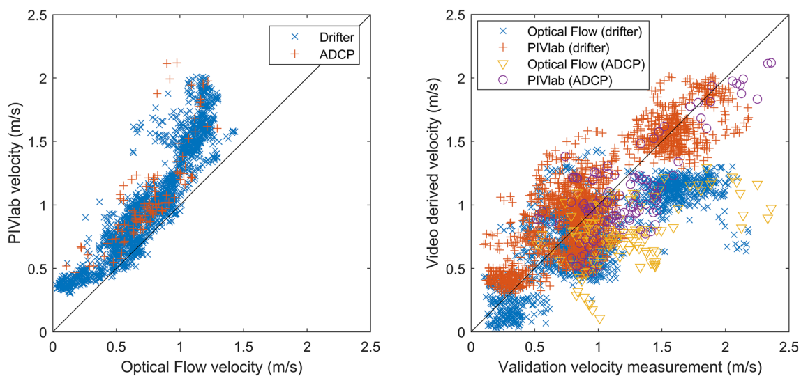
Fig. 6 Comparison between optical flow derived speeds and PIVlab derived speeds at validation data points for the Ramsey Sound dataset (left); comparison between validation velocity measurements
