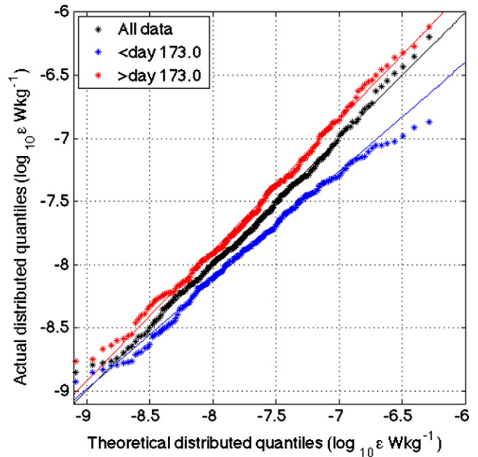
Fig. 11. QQ-plot of \log_{10} \varepsilon_{pyc} . Each point represents the quantiles estimated from the data, the lines show the equivalent representation of a log-normal distribution. While data from the entire period (black) is well described, we observe differing levels of agreement for data collected before (blue) and after (red) the energetic period occurring on day 173.
