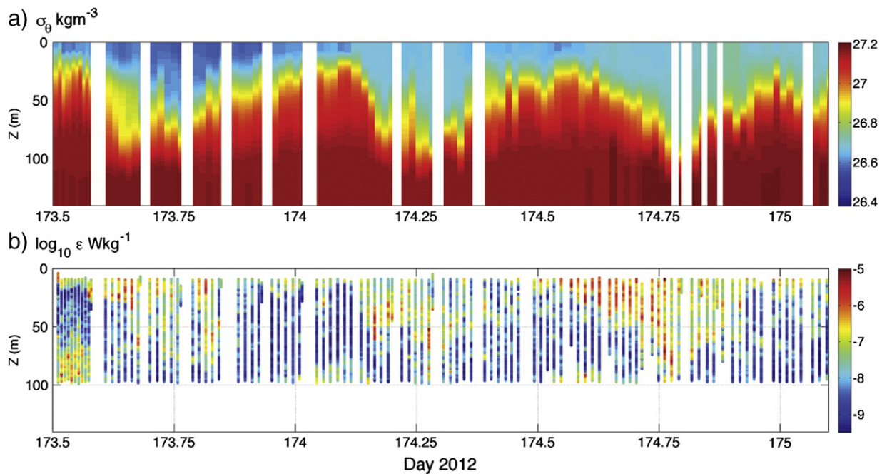
Fig. 8. (a) Density structure and (b) \log_{10} \varepsilon are shown for the most energetic period of the deployment. Three consecutive high-amplitude internal waves are characterized by high levels of turbulence in the ocean interior. Near surface turbulence appears to be drawn into the interior by vertical wave motion and pycnocline turbulence is also high and is often distinguishable from SML maxima.
