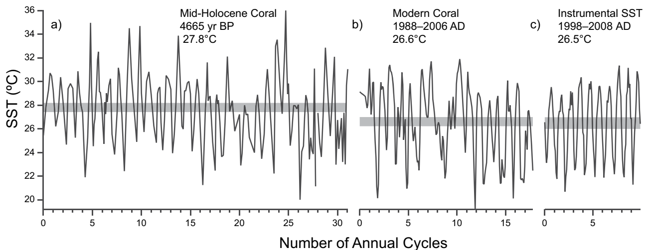
Figure 8. Temperature records from (a) mid-Holocene Sr/Ca derived record from KR-AMA-2, (b) modern microatoll KR-MMA-I Sr/Ca record, and (c) instrumental data obtained from Mourilyan Harbour in situ data logger ( http://www.aims.gov.au ). Temperature values given are the mean of each dataset, with gray shading indicating the 95% confidence interval of the mean.
