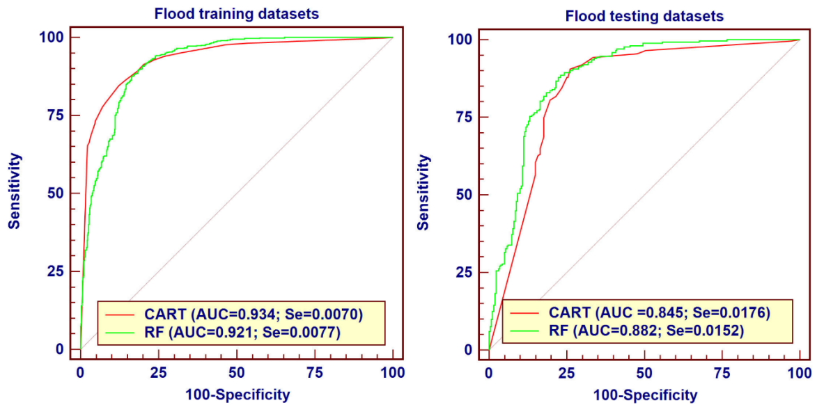
Figure 4. ROC curve and AUC analysis result from flood susceptibility modelling with training and validation datasets
