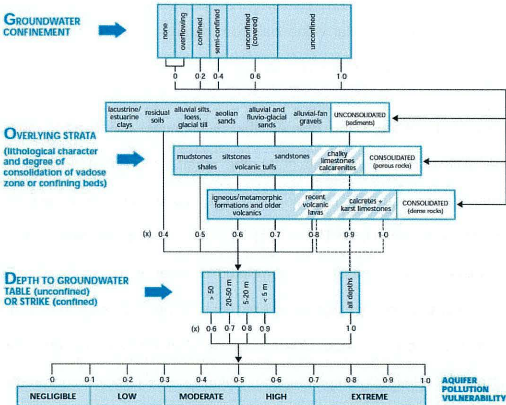
Figure 33. GOD scheme used to determine aquifer vulnerability to pollution by Foster, et al. (2002).
