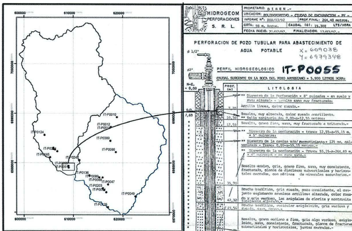
Figure 30. Diagram showing an example reading of the vadose zone type and the location of wells used to determine impact of the vadose zone media (I) in the watersheds.
