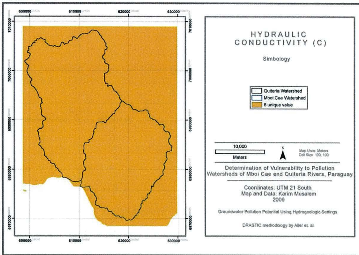
Figure 32. DRASTIC ratings for hydraulic conductivity (C) used in the determination of aquifer vulnerability to pollution in the Watersheds of the Mboi Cae and Quiteria Rivers, Paraguay.
