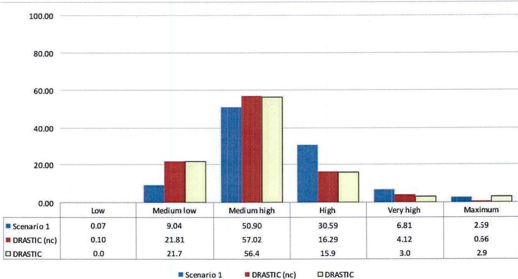
Figure 48. Comparative graph of DRASTIC ratings using: pesticide DRASTIC with predictive worst case scenario (rising of 5 meter change in water table; pesticide DRASTIC-nc (cities not considered as direct pollution sources); and pesticide DRASTIC (cities considered highest vulnerability values). Percent of area in the Watersheds of the Mboi Cae and Quiteria Rivers.
