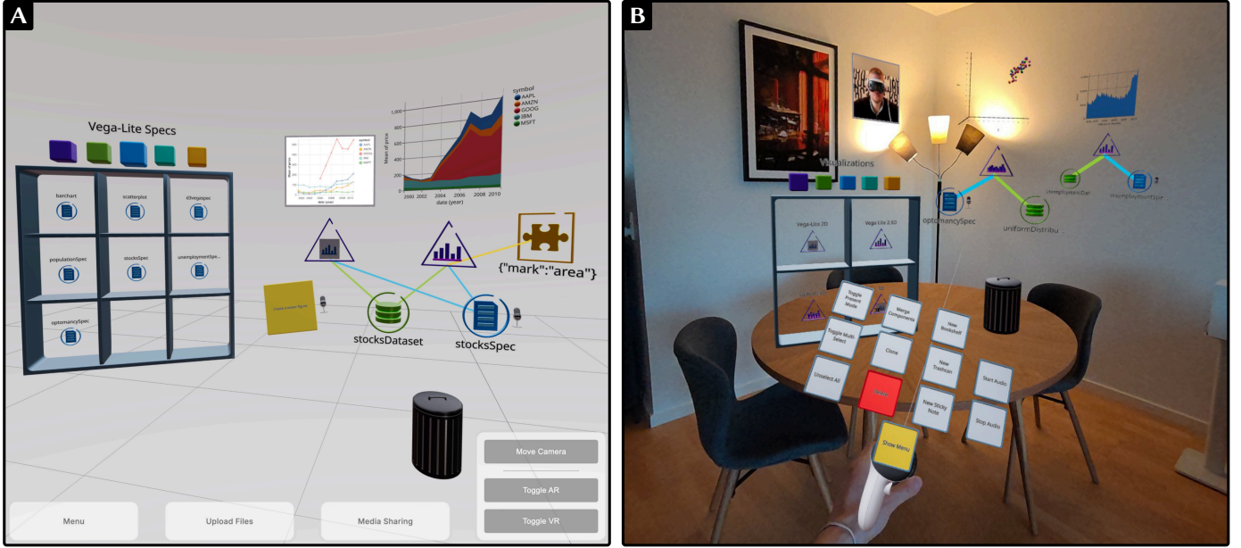
Fig. 2: DashSpace on Desktop and HMD. (A) The bookshelf showing available Vega-Lite specs in the library. A 2D and 2.5D visualization connected to the same dataset and spec; the latter is connected to a snippet that changes the mark type. A sticky note is visible in the center. (B) The bookshelf shows available visualization types as well as a 3D Optomancy and a 2.5D Vega-Lite visualization. The controller menu is visible in the foreground; in the background, a virtual image has been placed on the wall besides the physical one.
