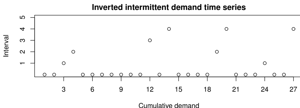
Figure 3: Inverted intermittent demand series.
